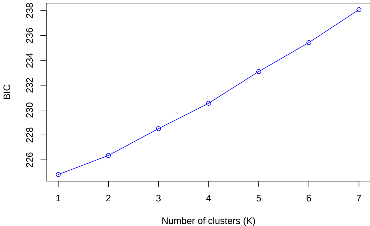
Value of BIC versus number of clusters WBNP: 1986 – 1999
