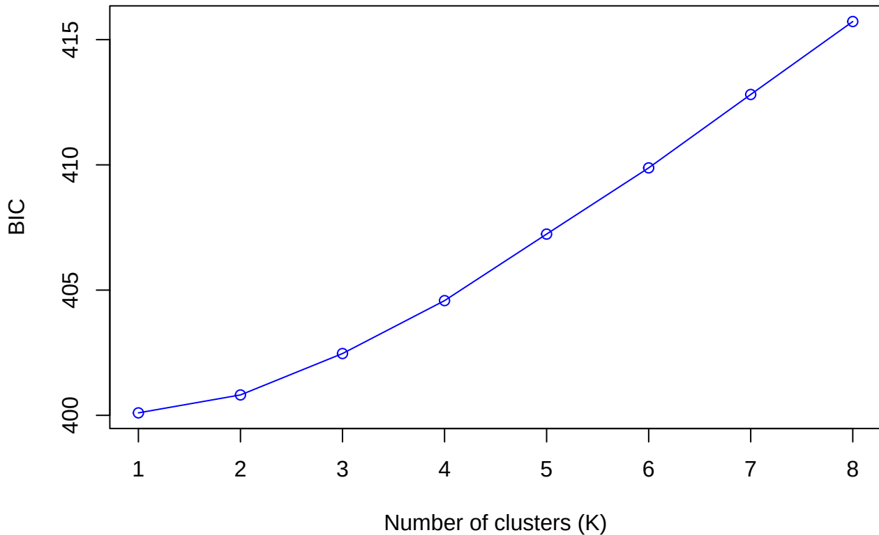
Value of BIC versus number of clusters WBNP: 2016 – 2025
