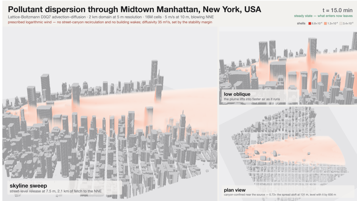
Figure 12: Midtown Manhattan at steady state, fifteen minutes into a continuous street-level release. Three shells of concentration, at the levels enclosing 95%, 80% and 50% of the plume’s mass — chosen from this frame rather than carried over from another run, since the same release spread over 2 km carries an order of magnitude less than it does over 200 m. Left: the skyline broadside to the plume, which runs left to right along the avenues. Top right: the same view from street level, showing the release threading between the towers. Bottom right: plan view, with the Commissioners’ grid visible; the wind bearing was measured out of the height field, not looked up. Every figure in the caption strip is read from the run’s own log, and the plan-view line is measured from this frame. The animation is doc/fig/manhattan_dispersion.mp4 .
