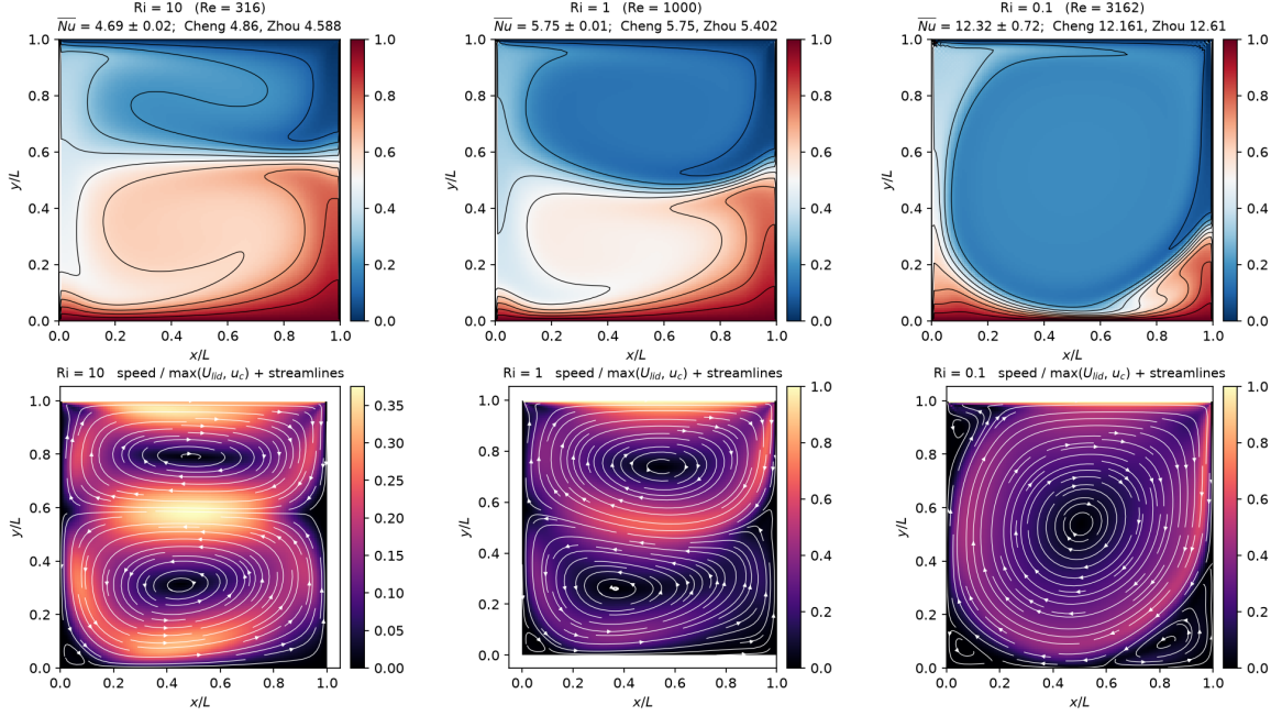
Figure 10: Thermal lid-driven cavity , Gr = 10^6 , Pr = 0.71 . Top: the temperature field with isotherms at \Delta\theta = 0.1 . Bottom: the speed with streamlines. Compare with the paper's Fig. 23 — two counter-rotating vortices stacked vertically with the lower one larger and a secondary vortex in the lower-left corner at Ri = 10 ; two of comparable strength at Ri = 1 ; a single primary vortex with three corner vortices at Ri = 0.1 . Rendered by doc/fig/zhou_lid_cavity.py .
