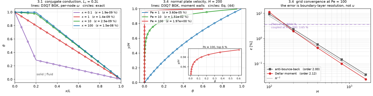
Figure 7: The two cases with exact solutions. Left: conjugate conduction, four conductivity ratios, against the piecewise linear steady state; the kink is the material interface at x/L = 0.2 . Centre: the normal-plate profile at Pe = 1, 10, 100 against Eq. (44), with the top six per cent inset because at Pe = 100 that is where the entire profile lives. Right: the refinement ladder, second order in both wall families, with the coupled framework’s 3.65% at H = 200 marked for scale. Rendered by doc/fig/zhou_analytic.py .
