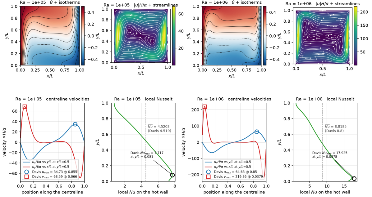
Figure 8: Natural convection in a square cavity , Ra = 10^5 and 10^6 . Top: the temperature field with isotherms, and the speed with streamlines. Bottom: the two centreline velocity profiles and the local Nusselt number on the hot wall, with de Vahl Davis's tabulated peaks marked — they land on the curves. Rendered by doc/fig/zhou_natural_convection.py .
