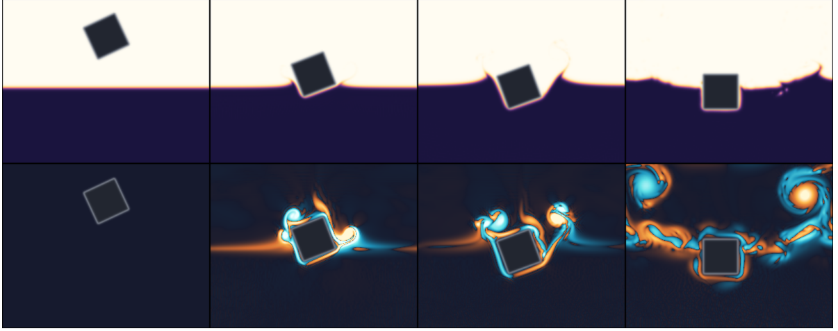
Figure 23: Water entry of a square at 0.6 times the water's density, released at 25^\circ from one body width above the surface; L = 48 , density ratio 50, \text{Re} = 2000 . Phase field above, out-of-plane vorticity below, at tU/L = 0, 2.4, 3.3 and 16.0 . The square strikes on one corner, sheds vortices of opposite sign from the two corners — the imbalance between them is what turns it — sinks past its draft, and returns upright and floating. A body lighter than the fluid it displaces is the case the classical fictitious-mass arrangement cannot express at all (§10.7).
