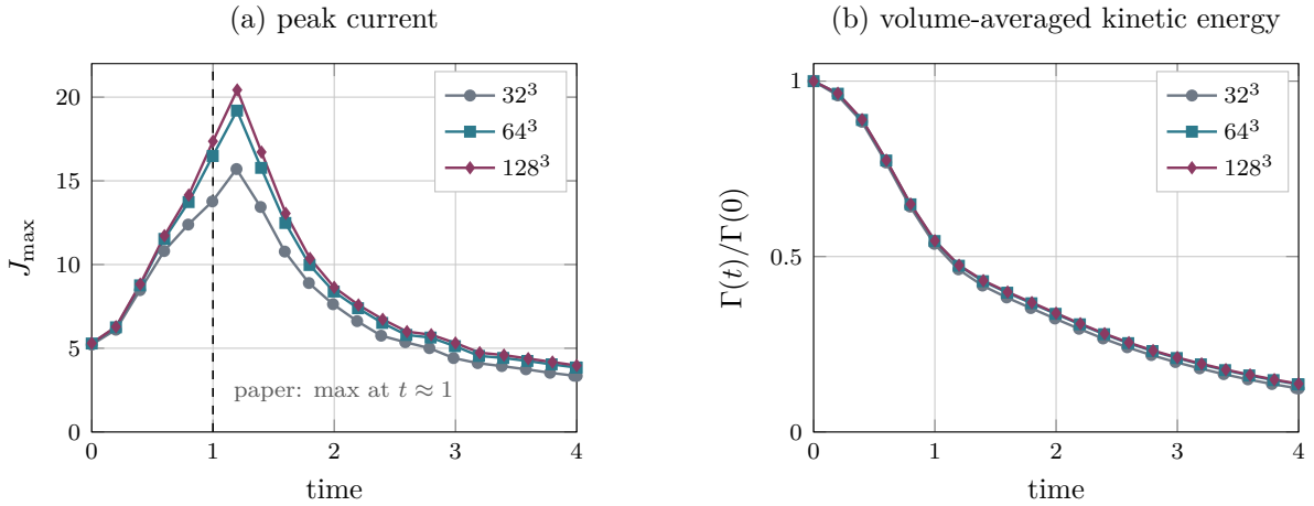
Figure 13: Three-dimensional Orszag–Tang vortex, D3Q27 with central moments, to be read against Fig. 6 of [13]. (a) The peak current magnitude rises with resolution as the current sheet is resolved, and its maximum converges to t = 1.200 against the paper’s stated t \approx 1 ; the value on the finest grid, 20.4, sits inside that figure’s 5–25 axis. (b) The energy, normalised as the paper normalises it, falls from 1 to 0.137. Both panels use a linear time axis; the published figure uses a logarithmic one.
