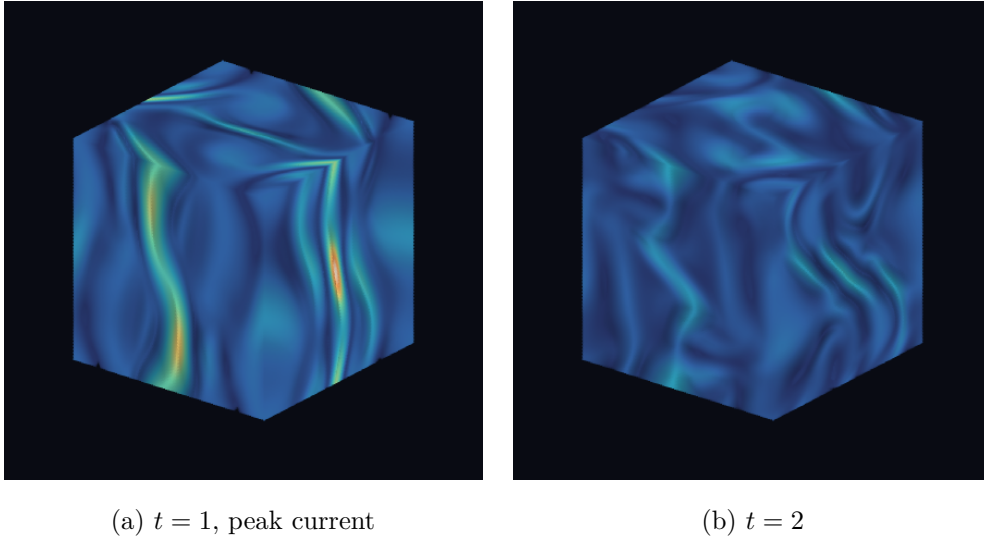
Figure 14: Three-dimensional Orszag–Tang vortex , current magnitude |\nabla \times \mathbf{b}| through the whole 128^3 box, D3Q27 with D3Q7 induction (§12.4.3). Volume rendered rather than sliced: a cut plane shows the sheets only where they happen to intersect it and says nothing about how they are oriented, which for this flow is the point. The current organises into curved sheets wrapping the box, and (a) is the instant the peak is reached — the same t \approx 1 the J_{\max} curve of Fig. 13 locates. Both panels share one colour scale , set by the t = 1 peak, so the visible dimming from (a) to (b) is the real decay: J_{\max} falls from 19.1 to 8.32, less than half, in the same units as Fig. 13. Normalising each panel to its own maximum — the default in most rendering tools — would have made the later, weaker field the brighter of the two. The reference is recomputed at this resolution rather than carried over from the 64^3 volumes: the raw lattice values differ between the two by the factor \Delta t \propto 1/M alone, so reusing the coarse-grid number would have rescaled the pair by about two. Orthographic view, azimuth 38^\circ , elevation 24^\circ ; emission–absorption compositing with the weak field left transparent, the local gradient used as a surface normal for a diffuse term so the sheets read as surfaces rather than fog, and 2\times supersampling. Rendered by doc/fig/vol3d.py , which is self-contained.
