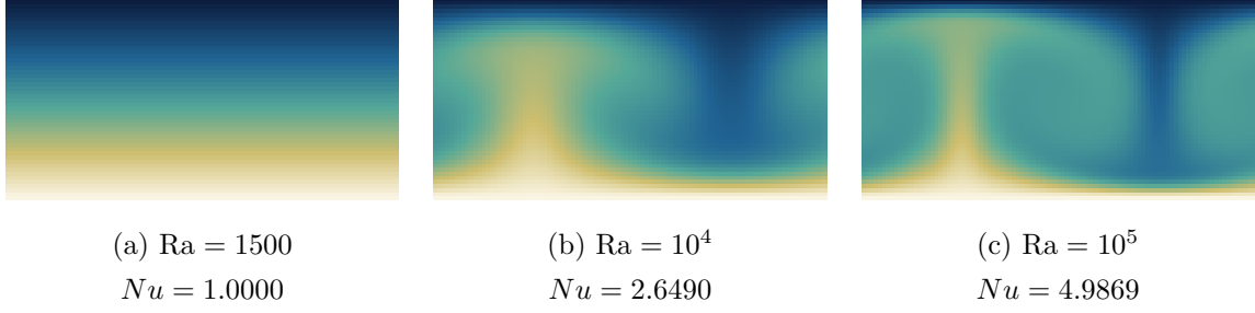
Figure 6: Rayleigh–Bénard convection , temperature, H = 48 , one critical wavelength wide, D2Q9 fluid with a D2Q5 scalar (§12.3.4). The three panels are the same run at three Rayleigh numbers and show what the Nusselt column of that section measures. (a) is below the critical Ra_c = 1707.762 : the perturbation decays and the field relaxes to pure conduction — a linear vertical gradient, no horizontal structure, and Nu = 1 to 6 \times 10^{-13} . (b) is supercritical, and the same perturbation grows into a steady convection cell with a hot plume rising against cold fluid descending. By (c), at 58.6 Ra_c , the thermal boundary layers at the two plates have thinned and the core is nearly isothermal — which is the mechanism behind Nu rising to 4.99, since Nu is precisely the wall gradient normalised by the conductive one. All three share a colour scale.
