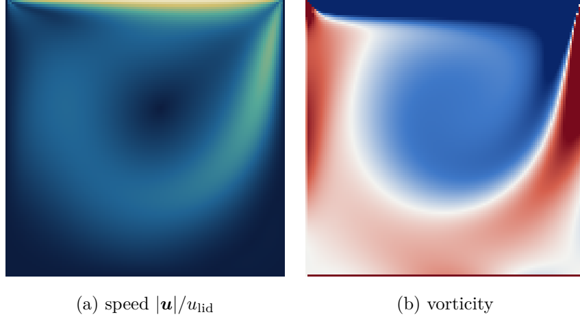
Figure 5: Lid-driven cavity at \text{Re} = 400, 129^2 , D2Q9 central moments, the run scored against Ghia et al. in §12 ( \max |\Delta u| = 0.0069 ). The primary vortex sits above and right of centre and both downstream corner eddies are resolved. The vorticity is clipped hard, at the 88th percentile against a peak twenty times larger, because it is concentrated in the lid boundary layer; without that the interior is blank.
