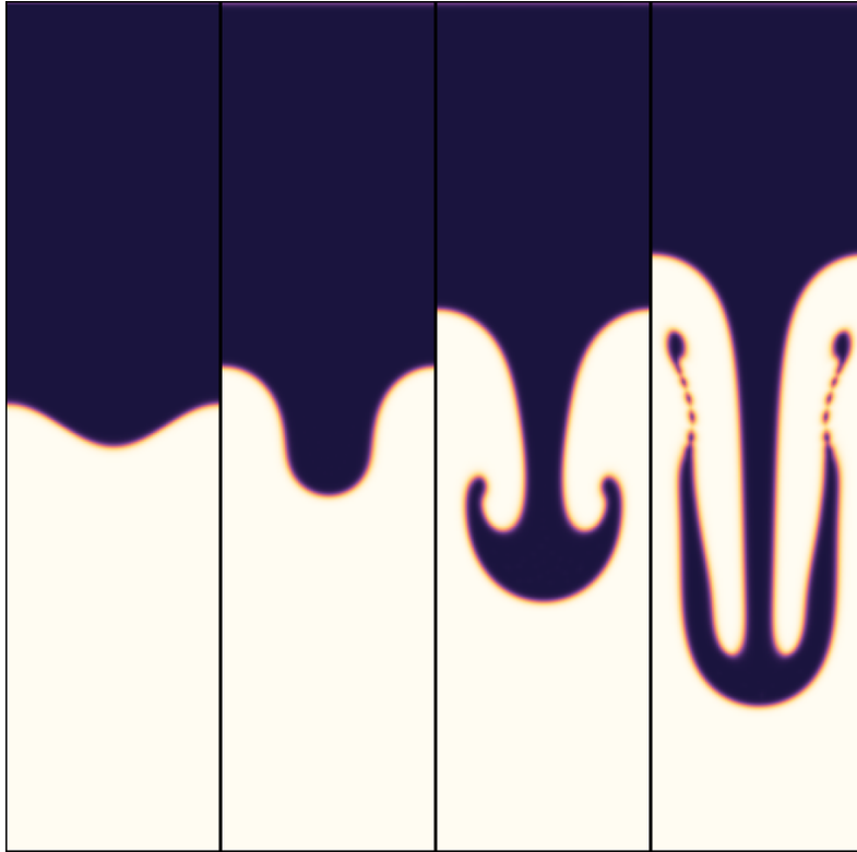
Figure 16: Rayleigh–Taylor instability at At = 0.5 , Re = 256 , W = 128 , central-moment operator. Phase field at t^* = 0, 1, 2 and 3 . The single-mode perturbation steepens into a falling spike, the spike rolls up into a mushroom, and by t^* = 3 the stem has gone secondarily unstable — the beads along it are Kelvin–Helmholtz billows on the shear between the descending spike and the rising fluid beside it. Nothing here is a measurement; what it shows is an interface that rolls up, reconnects and keeps going without the phase field being reinitialised.
