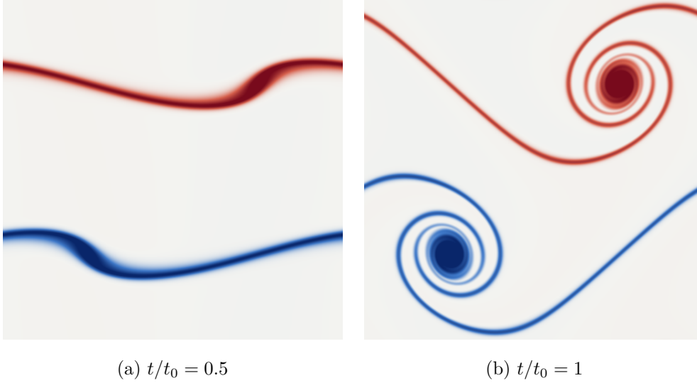
Figure 4: Double shear layer , vorticity, L = 512 , \text{Re} = 30\,000 , D2Q9 central moments (§12). By (a) the perturbation has begun to distort the two layers; by (b) each has rolled into a vortex, and the two are joined by a single unbroken braid. That the braid stays thin and connected is the whole test: at \tau = 0.50102 the flow is barely resolved, and an under-dissipative or unstable scheme shows it here first, by fragmenting the braid into secondary vortices that are numerical rather than physical. Doubling the resolution from the L = 256 of the campaign table sharpens the structure and, more usefully, quantifies the numerical dissipation: the enstrophy retained at t/t_0 = 1 rises from 0.6227 to 0.6432, and the energy from 0.98644 to 0.98696. The physical dissipation at this Reynolds number is negligible over one turnover, so nearly all of that difference is the scheme’s own, and it shrinks with resolution as it should. Colour saturates at the 99th percentile of |\zeta| .
