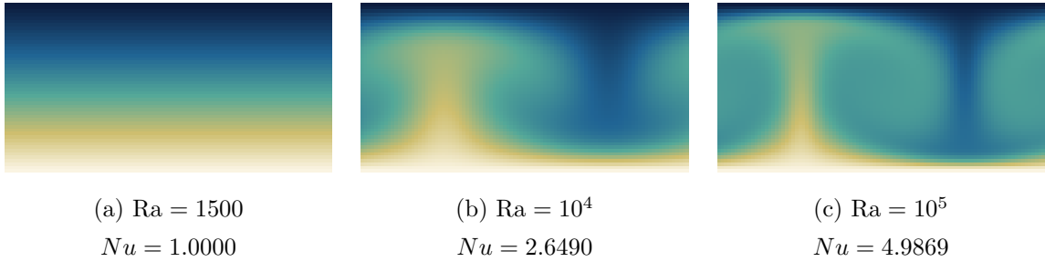
Figure 7: Rayleigh–Bénard convection , temperature, H = 48 , one critical wavelength wide, D2Q9 fluid with a D2Q5 scalar (§11.8). The three panels are the same run at three Rayleigh numbers and show what the Nusselt column of that section measures. (a) is below the critical \text{Ra}_c = 1707.762 : the perturbation decays and the field relaxes to pure conduction — a linear vertical gradient, no horizontal structure, and Nu = 1 to 6 \times 10^{-13} . (b) is supercritical, and the same perturbation grows into a steady convection cell with a hot plume rising against cold fluid descending. By (c), at 58.6 \text{ Ra}_c , the thermal boundary layers at the two plates have thinned and the core is nearly isothermal — which is the mechanism behind Nu rising to 4.99, since Nu is precisely the wall gradient normalised by the conductive one. All three share a colour scale.
