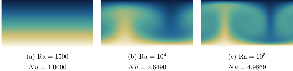
Figure 5: Rayleigh–Bénard convection , temperature, H = 48 , one critical wavelength wide, D2Q9 fluid with a D2Q5 scalar (§12.3.4). The three panels are the same run at three Rayleigh numbers and show what the Nusselt column of that section measures. (a) is below the critical Ra_c = 1707.762 : the perturbation decays and the field relaxes to pure conduction — a linear vertical gradient, no horizontal structure, and Nu = 1 to 6 \times 10^{-13} . (b) is supercritical, and the same perturbation grows into a steady convection cell with a hot plume rising against cold fluid descending. By (c), at 58.6 Ra_c , the thermal boundary layers at the two plates have thinned and the core is nearly isothermal — which is the mechanism behind Nu rising to 4.99, since Nu is precisely the wall gradient normalised by the conductive one. All three share a colour scale.
