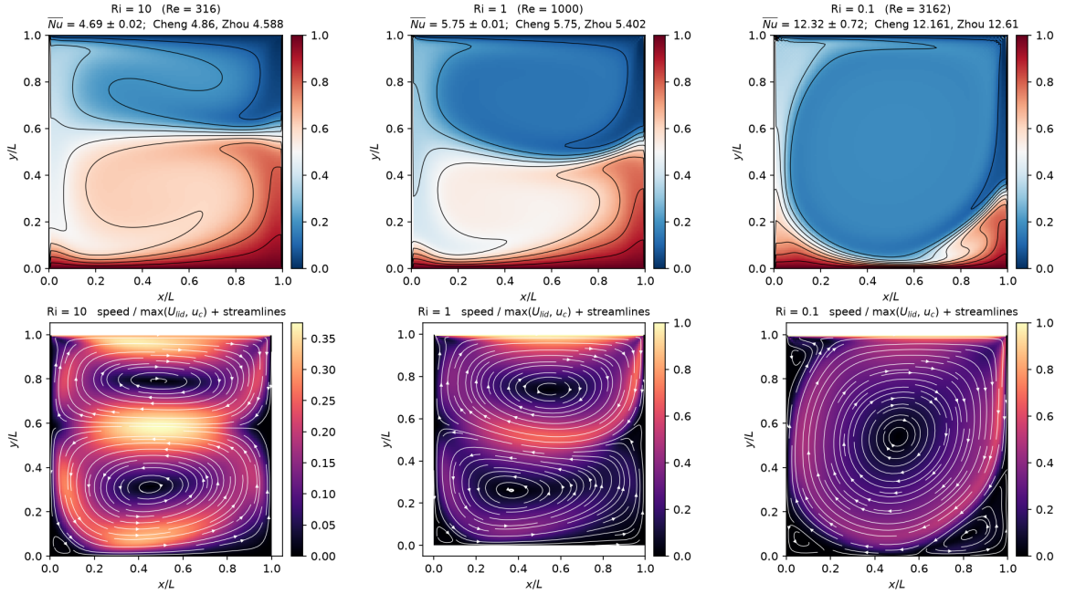
Figure 9: Thermal lid-driven cavity , Gr = 10^6 , Pr = 0.71 . Top: the temperature field with isotherms at \Delta\theta = 0.1 . Bottom: the speed with streamlines. Compare with the paper's Fig. 23 — two counter-rotating vortices stacked vertically with the lower one larger and a secondary vortex in the lower-left corner at Ri = 10 ; two of comparable strength at Ri = 1 ; a single primary vortex with three corner vortices at Ri = 0.1 . Rendered by doc/fig/zhou_lid_cavity.py .
