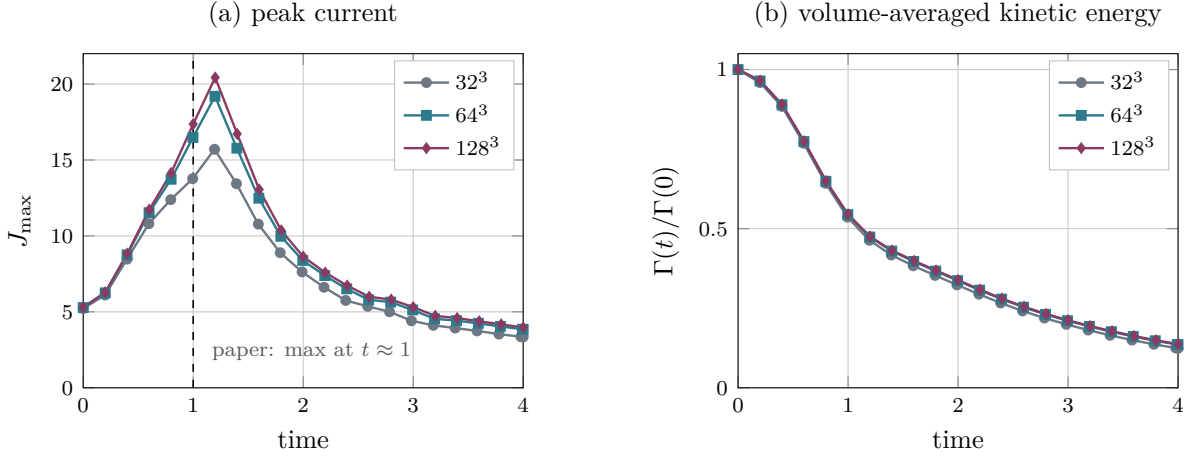
Figure 12: Three-dimensional Orszag–Tang vortex, D3Q27 with central moments, to be read against Fig. 6 of [13]. (a) The peak current magnitude rises with resolution as the current sheet is resolved, and its maximum converges to t = 1.200 against the paper’s stated t \approx 1 ; the value on the finest grid, 20.4, sits inside that figure’s 5–25 axis. (b) The energy, normalised as the paper normalises it, falls from 1 to 0.137. Both panels use a linear time axis; the published figure uses a logarithmic one.
