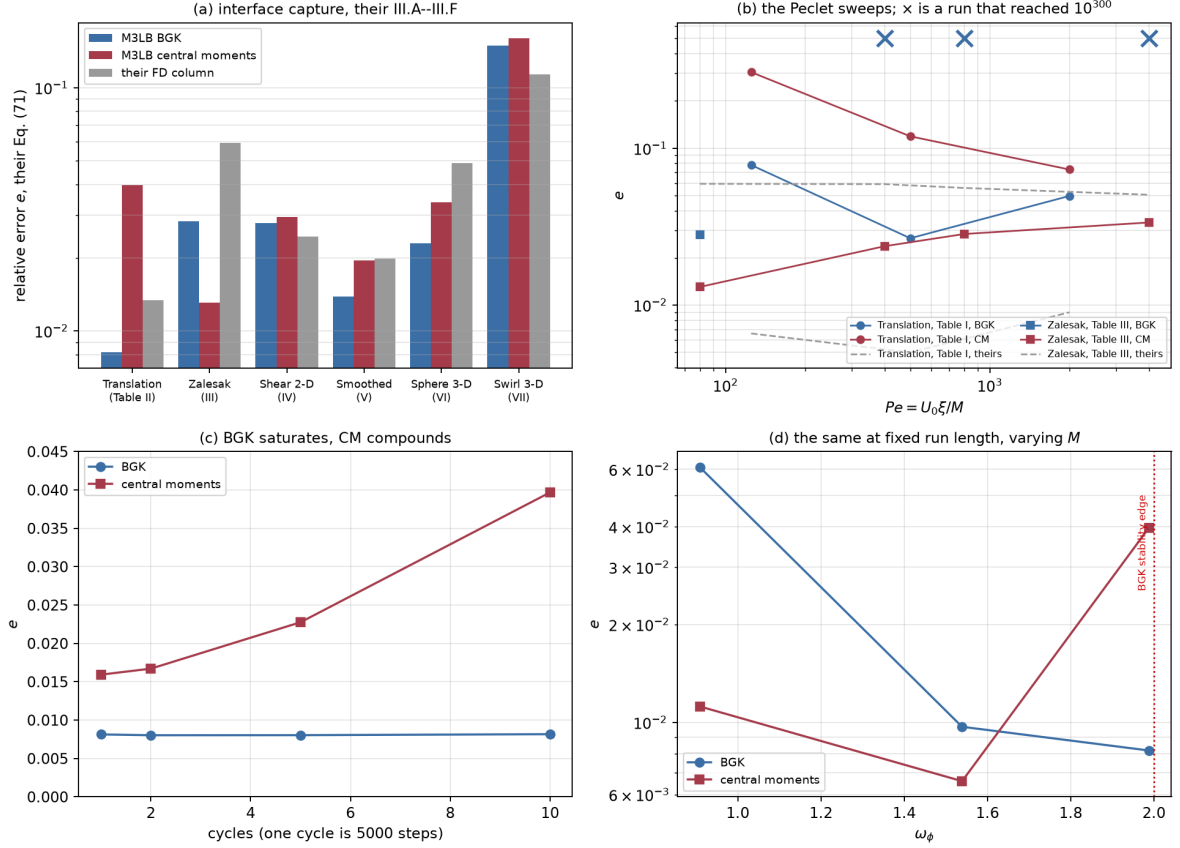
Figure 5: The interface-capture campaign. (a) the six cases of their III.A–III.F, both collisions against their finite-difference column; note that the translation case is the one where the central-moment operator loses badly and the Zalesak disk the one where it wins. (b) their Tables I and III; a cross marks a run that reached 10^{300} , and the three of them are the reason the central-moment operator exists. (c) the cycle scan, which is the measurement that disproved a crossover in \omega_\phi : BGK’s translation error is flat across a tenfold change in run length and the central-moment error compounds. (d) the mobility ladder at fixed run length, which is what made the \omega_\phi reading look right in the first place.
