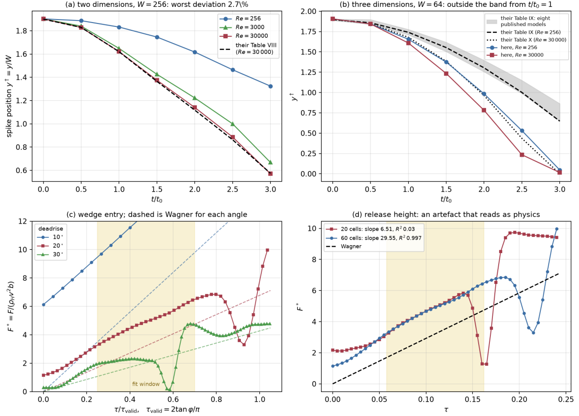
Figure 6: Rayleigh–Taylor and wedge entry. (a) the 2-D spike against their Table VIII at three Reynolds numbers — the pass. (b) the two 3-D cases against their Tables IX and X, with the band their Table IX collects from eight published models; being outside it from t/t_0 = 1 is the failure, drawn rather than asserted. (c) wedge entry at three deadrise angles with Wagner’s line for each and the fit window shaded; the 30^\circ curve collapsing inside the window has the same signature as (d) and is the same cause. (d) the release height: identical impact and window, and at 20 cells the pulse from the impulsive release returns inside the window and takes the fitted slope from 29.55 to 6.51.
