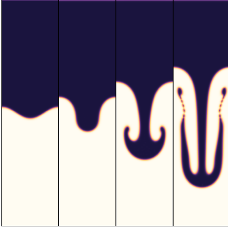
Figure 23: Rayleigh–Taylor instability at At = 0.5 , Re = 256 , W = 128 , central-moment operator. Phase field at t^* = 0, 1, 2 and 3 . The single-mode perturbation steepens into a falling spike, the spike rolls up into a mushroom, and by t^* = 3 the stem has gone secondarily unstable — the beads along it are Kelvin–Helmholtz billows on the shear between the descending spike and the rising fluid beside it. Nothing here is a measurement; what it shows is an interface that rolls up, reconnects and keeps going without the phase field being reinitialised.
