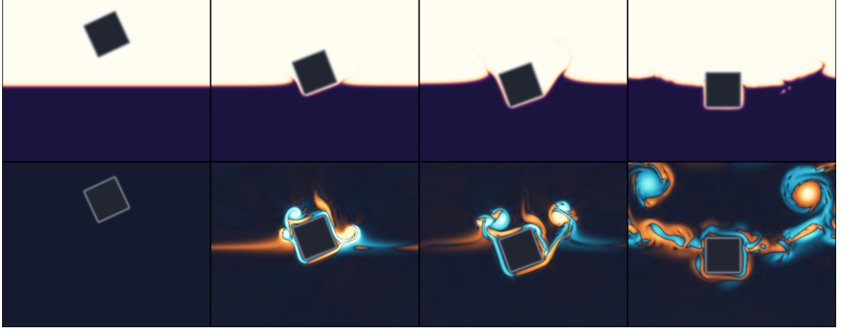
Figure 17: Water entry of a square at 0.6 times the water's density, released at 25^\circ from one body width above the surface; L = 48 , density ratio 50, \text{Re} = 2000 . Phase field above, out-of-plane vorticity below, at tU/L = 0, 2.4, 3.3 and 16.0 . The square strikes on one corner, sheds vortices of opposite sign from the two corners — the imbalance between them is what turns it — sinks past its draft, and returns upright and floating. A body lighter than the fluid it displaces is the case the classical fictitious-mass arrangement cannot express at all (§10.7).
