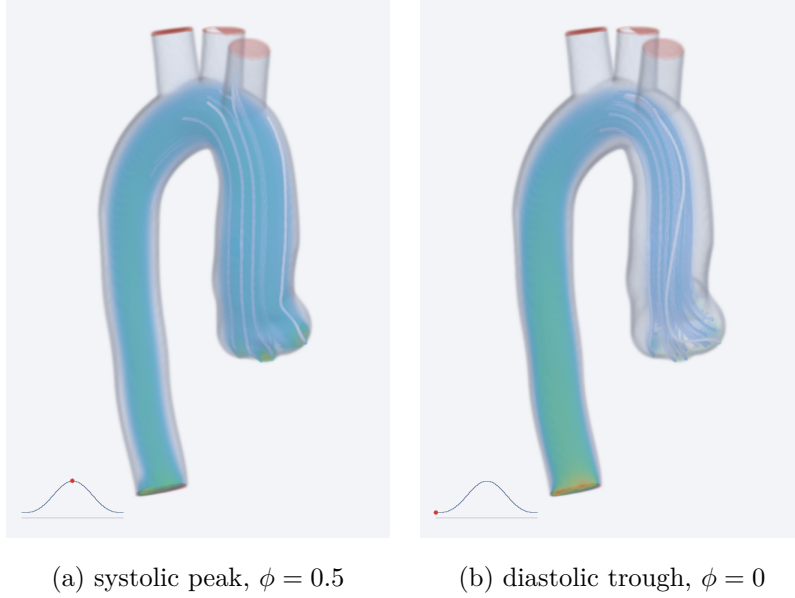
Figure 20: Pulsatile inflow , converged, \alpha = 7.05 , shared colour scale, with streamlines traced from the inlet cap through the current field. The inset traces (129) with a marker at the current phase. At systole the root drives a visible jet; at the diastolic trough it has gone pale while the descending aorta carries the fastest flow in the vessel — the antiphase fast tail of §13.4, which is a storage-and-release effect and not a Womersley lag. Both panels are from the same beat, at 3.8 viscous diffusion times, where every speed statistic repeats to every printed digit from beat to beat. The antiphase tail is quantitative, not an impression: at the trough p_{99.9} = 1.2317 \times 10^{-2} and |\mathbf{u}|_{\max} = 3.3362 \times 10^{-2} against 1.0446 \times 10^{-2} and 2.0743 \times 10^{-2} at the systolic peak, so the fastest fluid in the vessel is genuinely there when the inlet is slowest.
