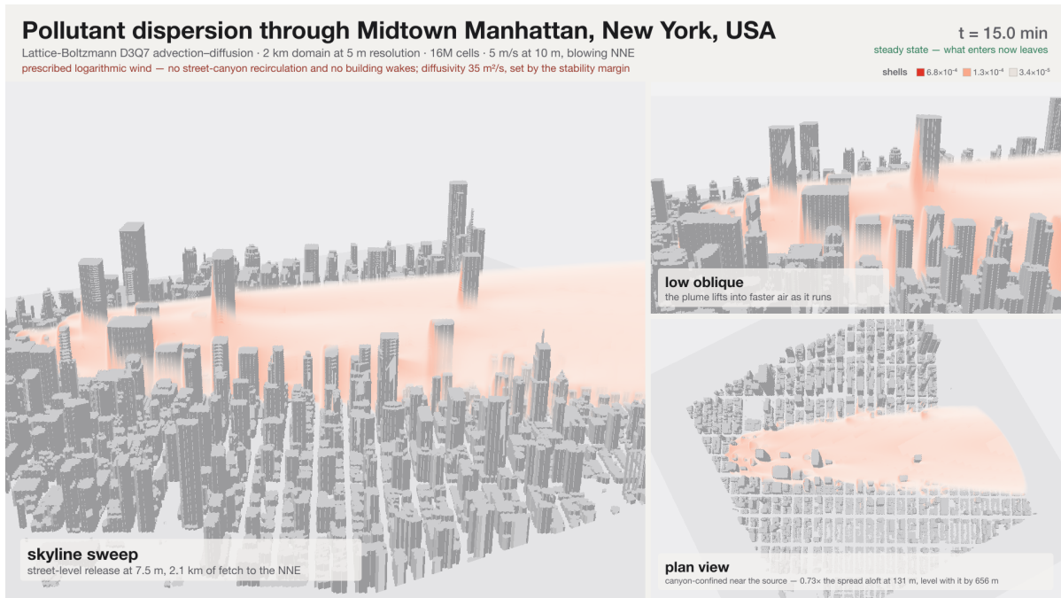
Figure 22: Midtown Manhattan at steady state, fifteen minutes into a continuous street-level release. Three shells of concentration, at the levels enclosing 95%, 80% and 50% of the plume's mass — chosen from this frame rather than carried over from another run, since the same release spread over 2 km carries an order of magnitude less than it does over 200 m. Left: the skyline broadside to the plume, which runs left to right along the avenues. Top right: the same view from street level, showing the release threading between the towers. Bottom right: plan view, with the Commissioners' grid visible; the wind bearing was measured out of the height field, not looked up. Every figure in the caption strip is read from the run's own log, and the plan-view line is measured from this frame. The animation is doc/fig/manhattan_dispersion.mp4 .
