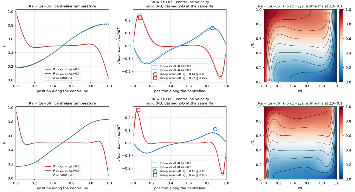
Figure 12: Cubic cavity , the same quantities the paper's Figs. 26–29 plot. Velocities are on the paper's own axis, u/u_{\text{ref}} with u_{\text{ref}} = \sqrt{g\beta h\Delta T} , which is exactly the u_c these runs are pinned with; the circles and squares are the Fusegi peaks read off those figures and are good to about five per cent. The dashed curves are the 2-D result at the same Rayleigh number. At Ra = 10^6 the u_x peak sitting well below its marker is the resolution shortfall discussed in the text, visible without needing the reference. Rendered by doc/fig/zhou_natural3d.py .
