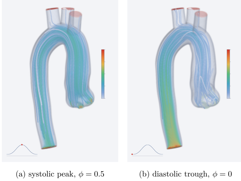
Figure 19: Pulsatile inflow , converged, \alpha = 8.04 , shared colour scale, with streamlines traced from the inlet cap through the current field. The inset traces (124) with a marker at the current phase. At systole the root drives a visible jet; at the diastolic trough it has gone pale while the descending aorta carries the fastest flow in the vessel — the antiphase fast tail of §13.4, which is a storage-and-release effect and not a Womersley lag. Both panels are from the same beat, at 2.9 viscous diffusion times, where every speed statistic repeats to eight significant figures from beat to beat.
