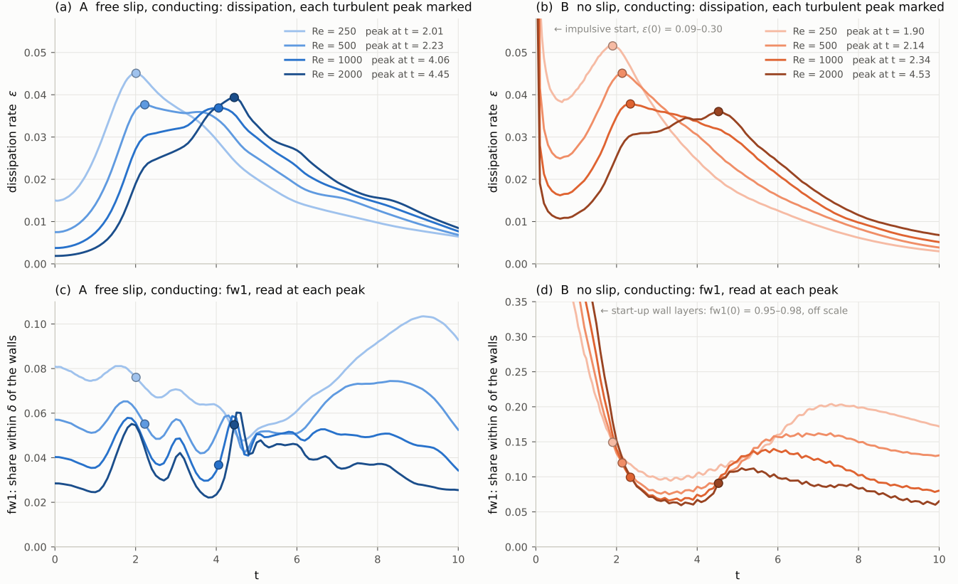
FIG. 5. The turbulent peak switches. The dissipation rate \epsilon(t) (a, b) and the share within \delta of the walls, f_1(t) (c, d), for the free-slip box A (a, c) and the no-slip box B (b, d) at Re = 250-2000 (light to dark). Dots mark each run's turbulent peak and the f_1 read there. A's early maximum is the larger up to Re = 500 and its later one from Re = 1000 ; B's switches between Re = 1000 and 2000 . B starts off scale at t = 0 (impulsive start).
