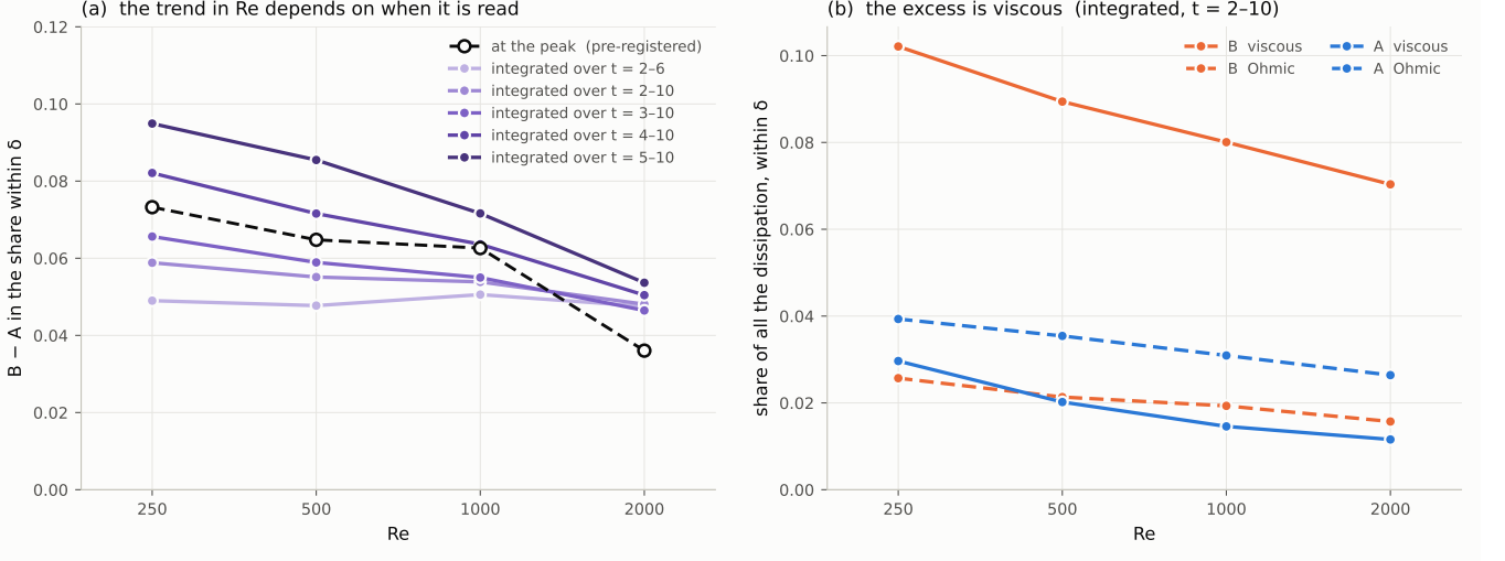
FIG. 2. (a) B–A in the share of the dissipation within \delta of the walls against Re: at the turbulent peak, as pre-registered (dashed), and integrated over five time windows, after the fact (light to dark: later windows). (b) The integrated share F_1 over t = 2-10 for A and B, divided into its viscous and Ohmic parts. Grid bands are at most 0.001, smaller than the symbols.
