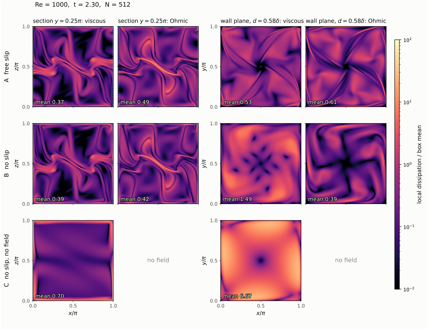
FIG. 3. Where the dissipation sits, at Re = 1000 and t = 2.3 (B's turbulent peak), on the finer grid ( N = 512 ). Rows: the free-slip box A, the no-slip box B and the box without a field C. Columns: the viscous and Ohmic dissipation, \nu|\omega|^2 and \eta|j|^2 , in the vertical section y = \pi/4 , with dashed lines at \delta from its four walls, and in the plane 0.58\delta above the bottom wall. One logarithmic colour scale, relative to each box's mean dissipation at that time; each panel gives its plane's mean.
