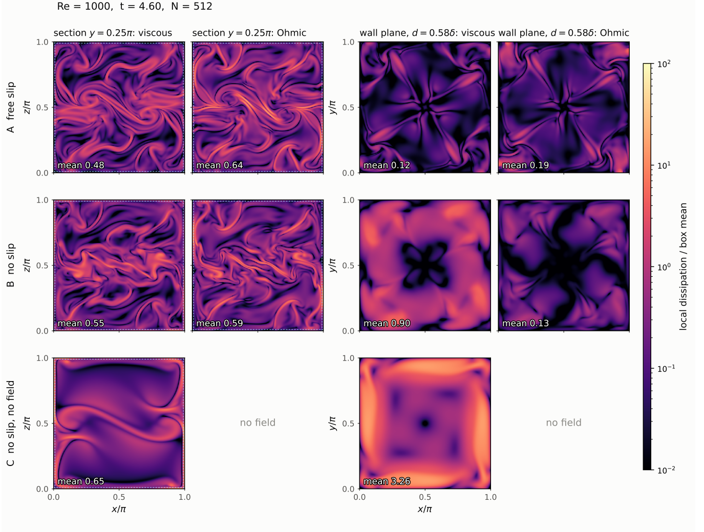
FIG. 4. As Fig. 3, at t = 4.6 , by the later maxima of the dissipation.
