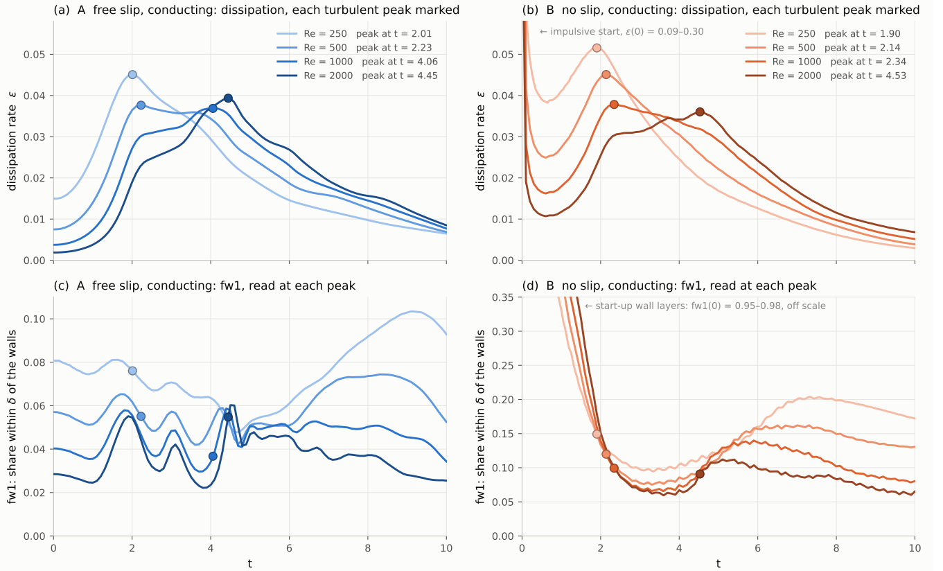
FIG. 2. The turbulent peak switches. The dissipation rate \epsilon(t) (a, b) and the share within \delta of the walls, f_1(t) (c, d), for the free-slip box A (a, c) and the no-slip box B (b, d) at Re = 250-2000 (light to dark). Dots mark each run's turbulent peak and the f_1 read there. A's early maximum is the larger up to Re = 500 and its later one from Re = 1000 ; B's switches between Re = 1000 and 2000 . B starts off scale at t = 0 (impulsive start).
