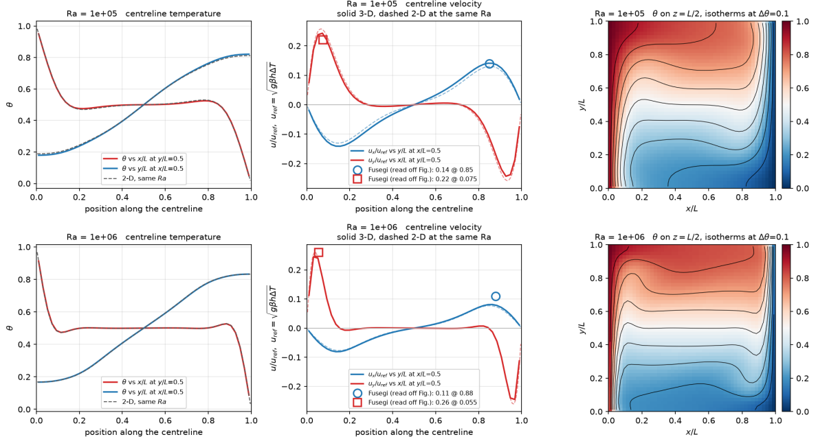
Figure 12: Cubic cavity, the same quantities the paper’s Figs. 26–29 plot. Velocities are on the paper’s own axis, u/u_{\text{ref}} with u_{\text{ref}} = \sqrt{g\beta h\Delta T} , which is exactly the u_c these runs are pinned with; the circles and squares are the Fusegi peaks read off those figures and are good to about five per cent. The dashed curves are the 2-D result at the same Rayleigh number. At \text{Ra} = 10^6 the u_x peak sitting well below its marker is the resolution shortfall discussed in the text, visible without needing the reference. Rendered by doc/fig/zhou_natural3d.py .
