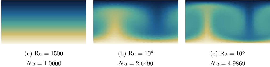
Figure 7: Rayleigh–Bénard convection , temperature, H = 48 , one critical wavelength wide, D2Q9 fluid with a D2Q5 scalar (§12.3.4). The three panels are the same run at three Rayleigh numbers and show what the Nusselt column of that section measures. (a) is below the critical Ra_c = 1707.762 : the perturbation decays and the field relaxes to pure conduction — a linear vertical gradient, no horizontal structure, and Nu = 1 to 6 \times 10^{-13} . (b) is supercritical, and the same perturbation grows into a steady convection cell with a hot plume rising against cold fluid descending. By (c), at 58.6 Ra_c , the thermal boundary layers at the two plates have thinned and the core is nearly isothermal — which is the mechanism behind Nu rising to 4.99, since Nu is precisely the wall gradient normalised by the conductive one. All three share a colour scale.
