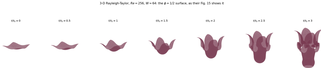
Figure 6: The \phi = 1/2 surface of the 3-D case at Re = 256 , the counterpart of their Fig. 15, extracted by marching cubes from the volumes validation/enan_rt -field -vol writes. The morphology is what their text describes — a mushroom-shaped spike, rising bubbles, and four saddle points at the middle of the four sides — which is why the disagreement in Table 8 is read as a rate rather than as a broken force.
