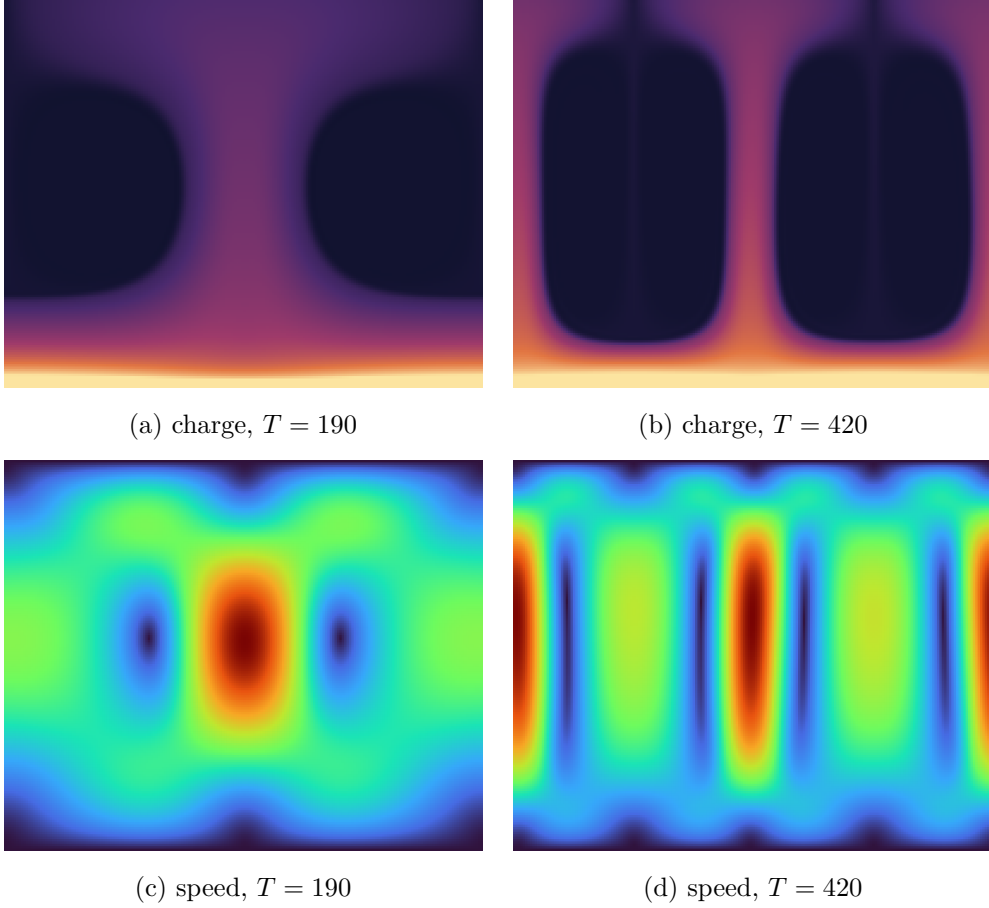
Figure 16: Electroconvection at C = 10 , M = 10 , A = 0.614 , n_y = 163 , D2Q9 fluid and charge with D2Q5 potential (§12.5.2). The box is periodic and twice the reference’s width; a free-slip wall is the mirror plane of a doubled periodic box, so each panel shows two of the reference’s cells. Charge is scaled to [0, 0.5 q_0] and saturates: the injector row is q = q_0 by construction, and the dark lobes are the charge-depleted void regions the reference reads as a hallmark of the subcritical bifurcation. Speed is scaled to its own peak, 3.76 u_0 in (c) and 4.43 u_0 in (d); its dark points are the vortex cores, two in (c) and four in (d). The change of lateral wavenumber between the columns — m = 1 to m = 2 — is measured, not imposed, and reproduces the reference’s description of a single cell at T = 190 becoming a counter-rotating pair at T = 420 .
