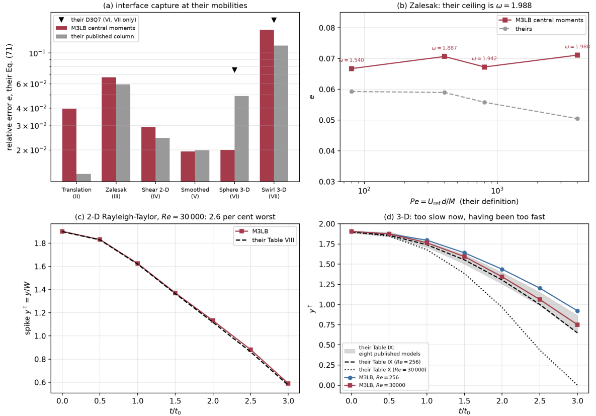
Figure 5: The campaign at their parameters, central moments throughout. (a) interface capture against the published column, with the D3Q7 entries their Tables VI and VII also give. (b) the Zalesak Peclet sweep with \omega_\phi marked: their domain-based mobility puts the ceiling at 1.988, and an earlier revision of this section read Pe as U_0 \xi / M , ran at 1.9998, and drew conclusions from a regime the paper never visits. (c) the 2-D Rayleigh–Taylor spike against their Table VIII — the pass. (d) the two 3-D cases against Tables IX and X, with the band their Table IX collects from eight published models; both now sit above it, having sat far below it before the reference time was corrected.
