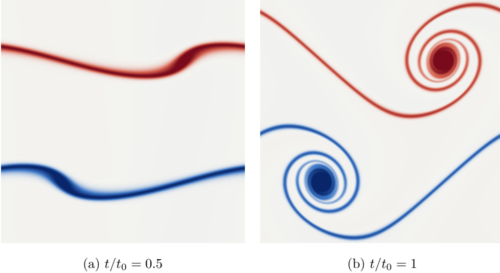
Figure 3: Double shear layer , vorticity, L = 512 , \text{Re} = 30\,000 , D2Q9 central moments (§12.1.6). By (a) the perturbation has begun to distort the two layers; by (b) each has rolled into a vortex, and the two are joined by a single unbroken braid. That the braid stays thin and connected is the whole test: at \tau = 0.50102 the flow is barely resolved, and an under-dissipative or unstable scheme shows it here first, by fragmenting the braid into secondary vortices that are numerical rather than physical. Doubling the resolution from the L = 256 of the campaign table sharpens the structure and, more usefully, quantifies the numerical dissipation: the enstrophy retained at t/t_0 = 1 rises from 0.6227 to 0.6432, and the energy from 0.98644 to 0.98696. The physical dissipation at this Reynolds number is negligible over one turnover, so nearly all of that difference is the scheme’s own, and it shrinks with resolution as it should. Colour saturates at the 99th percentile of |\zeta| .
