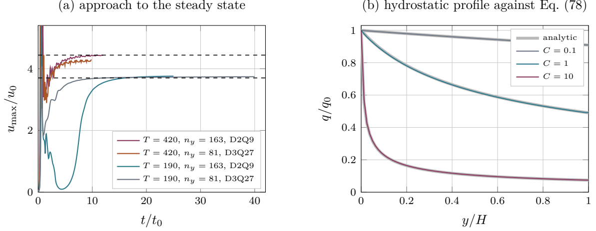
Figure 17: Electrohydrodynamics. (a) Peak velocity against time for the four production runs (§12.5.2); dashed lines are the reference’s converged values, 3.70 and 4.44. The T = 420 pair separates: D3Q27 converges 4.55% below D2Q9 at n_y = 81 , and refining brings D2Q9 down onto the published value. All four overshoot near t/t_0 \approx 1 before settling. (b) Hydrostatic charge profiles at H = 80 against the analytic solution (§12.5.1), thick grey.
