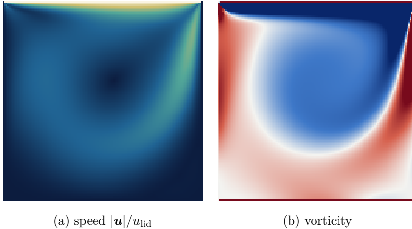
Figure 4: Lid-driven cavity at \text{Re} = 400 , 129^2 , D2Q9 central moments, the run scored against Ghia et al. in §12.1.6 ( \max |\Delta u| = 0.0069 ). The primary vortex sits above and right of centre and both downstream corner eddies are resolved. The vorticity is clipped hard, at the 88th percentile against a peak twenty times larger, because it is concentrated in the lid boundary layer; without that the interior is blank.
