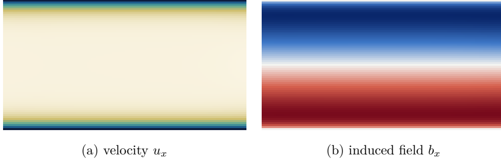
Figure 2: Inlet-driven Hartmann flow , \text{Ha} = 10 , L_y = 65 , D2Q9 fluid with D2Q5 induction, central moments (§12.1.5). The velocity shows the flat Hartmann core with boundary layers of thickness L/\text{Ha} ; the induced field is antisymmetric about the centreline, vanishing there and at both walls. Both are visibly independent of the streamwise coordinate, which is the property the exact solution has and which the convergence table depends on — any x structure here would be boundary error, and it is how the magnetic outflow defect (§8.7) was found.
