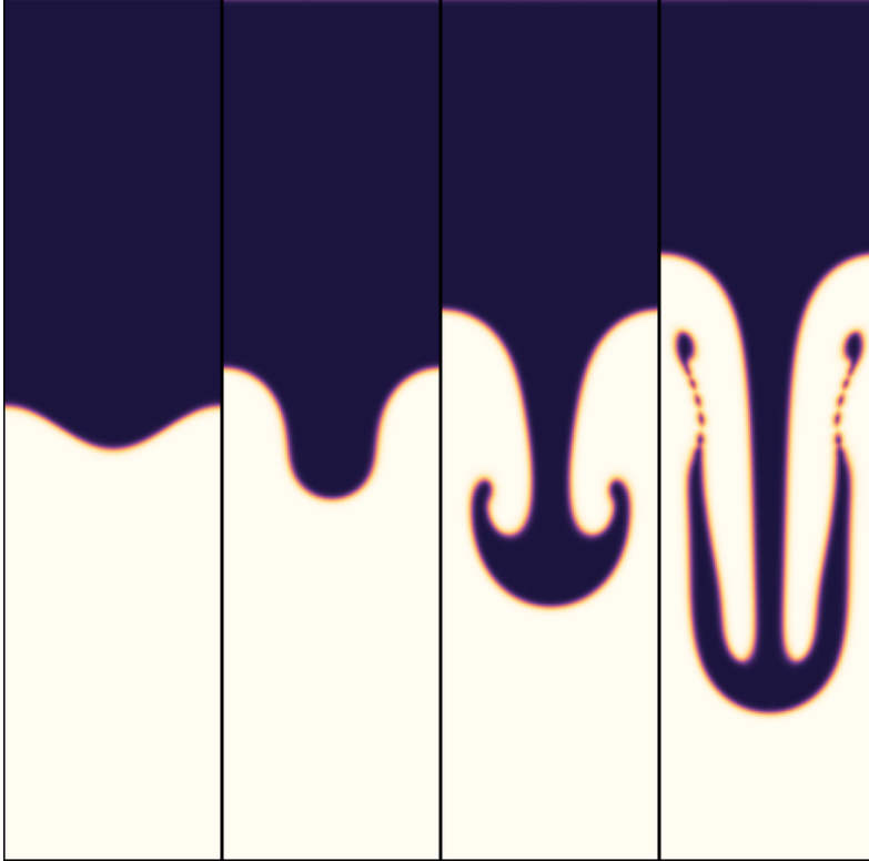
Figure 25: Rayleigh–Taylor instability at \text{At} = 0.5 , \text{Re} = 256 , W = 128 , central-moment operator. Phase field at t^* = 0, 1, 2 and 3 . The single-mode perturbation steepens into a falling spike, the spike rolls up into a mushroom, and by t^* = 3 the stem has gone secondarily unstable — the beads along it are Kelvin–Helmholtz billows on the shear between the descending spike and the rising fluid beside it. Nothing here is a measurement; what it shows is an interface that rolls up, reconnects and keeps going without the phase field being reinitialised.
