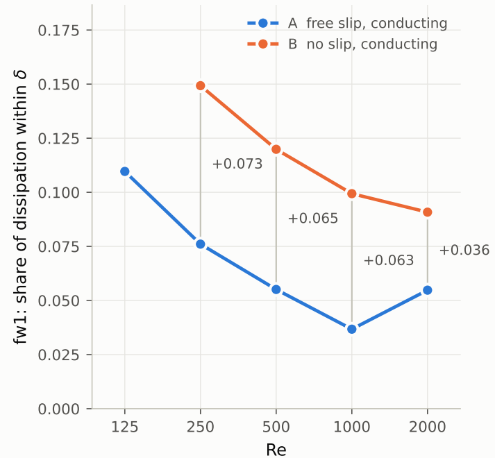
(c) pre-registered: fw1 at the peak ( B - A )
