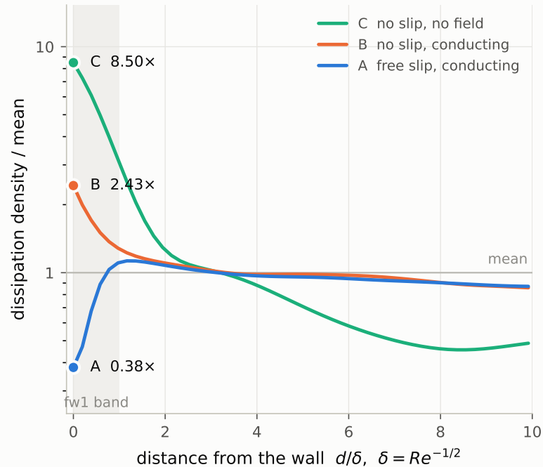
(a) where it dissipates, Re = 1000 , t = 2-10
