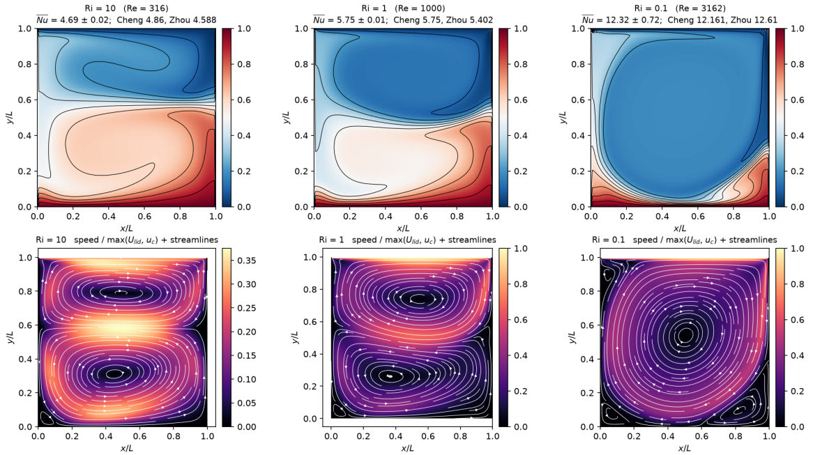
Figure 11: Thermal lid-driven cavity, Gr = 10^6 , Pr = 0.71 . Top: the temperature field with isotherms at \Delta\theta = 0.1 . Bottom: the speed with streamlines. Compare with the paper's Fig. 23 — two counter-rotating vortices stacked vertically with the lower one larger and a secondary vortex in the lower-left corner at Ri = 10 ; two of comparable strength at Ri = 1 ; a single primary vortex with three corner vortices at Ri = 0.1 . Rendered by doc/fig/zhou_lid_cavity.py .
