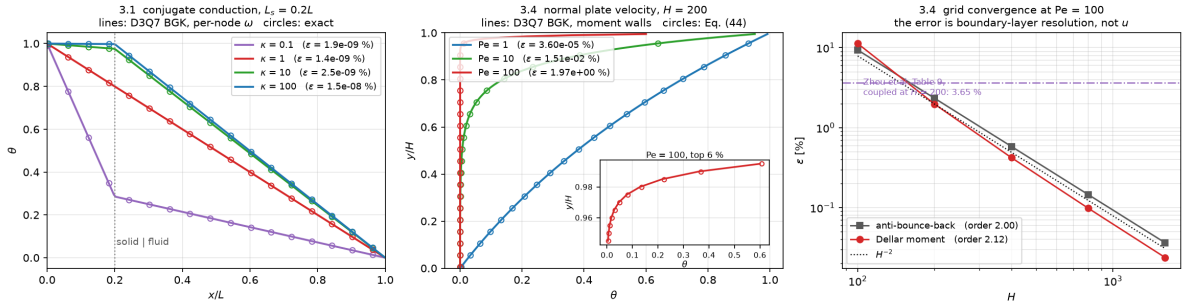
Figure 8: The two cases with exact solutions. Left: conjugate conduction, four conductivity ratios, against the piecewise linear steady state; the kink is the material interface at x/L = 0.2 . Centre: the normal-plate profile at \text{Pe} = 1, 10, 100 against Eq. (44), with the top six per cent inset because at \text{Pe} = 100 that is where the entire profile lives. Right: the refinement ladder, second order in both wall families, with the coupled framework’s 3.65% at H = 200 marked for scale. Rendered by doc/fig/zhou_analytic.py .
