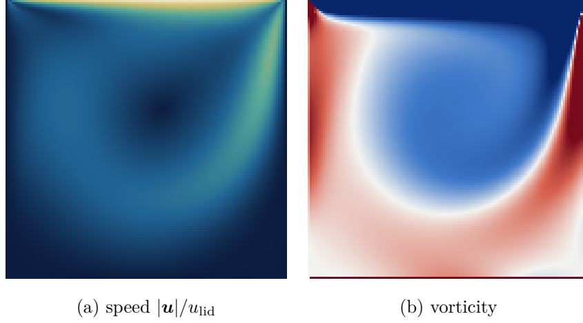
Figure 4: Lid-driven cavity at \text{Re} = 400, 129^2 , D2Q9 central moments, the run scored against Ghia et al. in §12.1.6 ( \max |\Delta u| = 0.0069 ). The primary vortex sits above and right of centre and both downstream corner eddies are resolved. The vorticity is clipped hard, at the 88th percentile against a peak twenty times larger, because it is concentrated in the lid boundary layer; without that the interior is blank.
