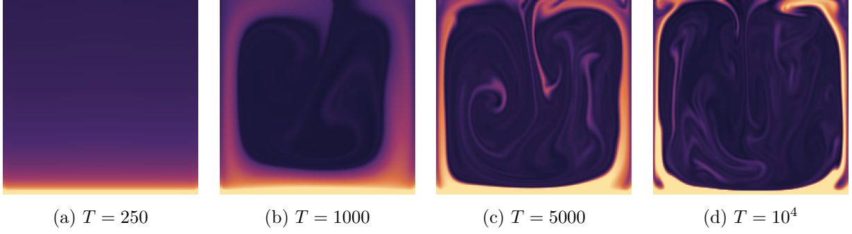
Figure 18: Closed square cavity: charge density q/q_0 at t/t_0 = 8 , 201 \times 201 , injector along the bottom edge (§12.5.3). Colour is linear on [0, 0.5 q_0] and saturates, as in Fig. 16. These are the four states of the reference’s Fig. 9 and they carry the features its text names individually: (a) a smooth diffusive layer with no electroconvective structure, the flow still hydrostatic; (b) a single coherent plume-like roll rising toward the centre, cleanly separated from the lateral layers; (c) multiple filaments and secondary vortices, with sharp gradients along the walls; (d) irregular plumes climbing both vertical walls, counter-rotating charge spirals in both upper corners, and a disordered, charge-depleted core. Panel (a) is run unseeded — with a seed the cavity convects at T = 250 , which is the branch selection discussed above — and (b)–(d) carry a 10^{-4}q_0 perturbation so the flow is developed inside the window.
