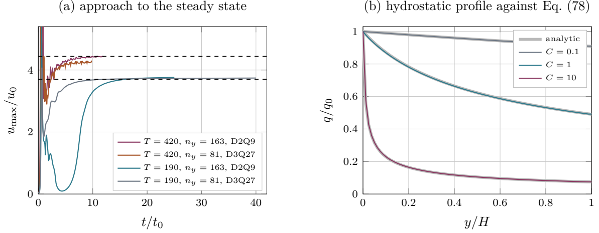
Figure 17: Electrodynamics. (a) Peak velocity against time for the four production runs (§12.5.2); dashed lines are the reference’s converged values, 3.70 and 4.44. The T = 420 pair separates: D3Q27 converges 4.55% below D2Q9 at n_y = 81 , and refining brings D2Q9 down onto the published value. All four overshoot near t/t_0 \approx 1 before settling. (b) Hydrostatic charge profiles at H = 80 against the analytic solution (§12.5.1), thick grey.
