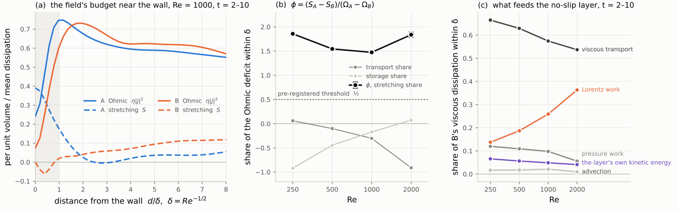
FIG. 6. What feeds the near-wall Ohmic dissipation, over t = 2-10 , on the finer grid of each rung. (a) At Re = 1000 , the stretching S = B_i B_j \partial_j v_i (dashed) and the Ohmic dissipation \eta|j|^2 (solid) per unit volume, relative to the box-mean dissipation, against d/\delta , for A and B; the shaded band is \delta . (b) \phi , the share of the near-wall Ohmic deficit that the stretching deficit accounts for [Eq. (11)], with its two-grid band, mostly smaller than the symbols, against the pre-registered threshold \frac{1}{2} ; the transport and storage shares are its complements, the three adding to one. (c) What supplies B's viscous dissipation within \delta , as shares of it.
