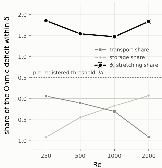
(b) \phi = (S_A - S_B)/(\Omega_A - \Omega_B)
