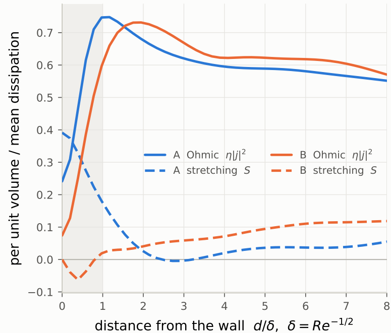
(a) the field's budget near the wall, Re = 1000 , t = 2-10
