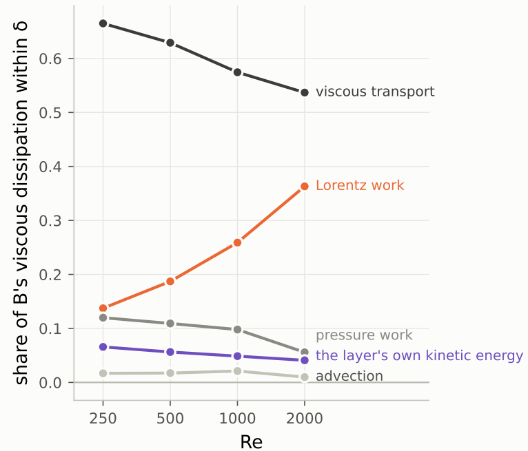
(c) what feeds the no-slip layer, t = 2-10
