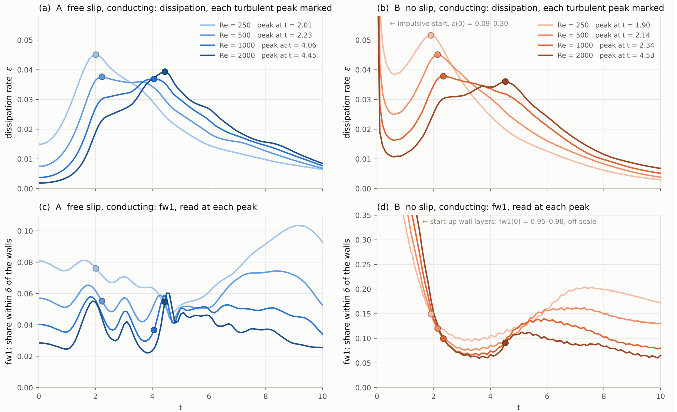
FIG. 3. The turbulent peak switches. The dissipation rate \epsilon(t) (a, b) and the share within \delta of the walls, f_1(t) (c, d), for the free-slip box A (a, c) and the no-slip box B (b, d) at Re = 250-2000 (light to dark). Dots mark each run's turbulent peak and the f_1 read there. A's early maximum is the larger up to Re = 500 and its later one from Re = 1000 ; B's switches between Re = 1000 and 2000 . B starts off scale at t = 0 (impulsive start).
