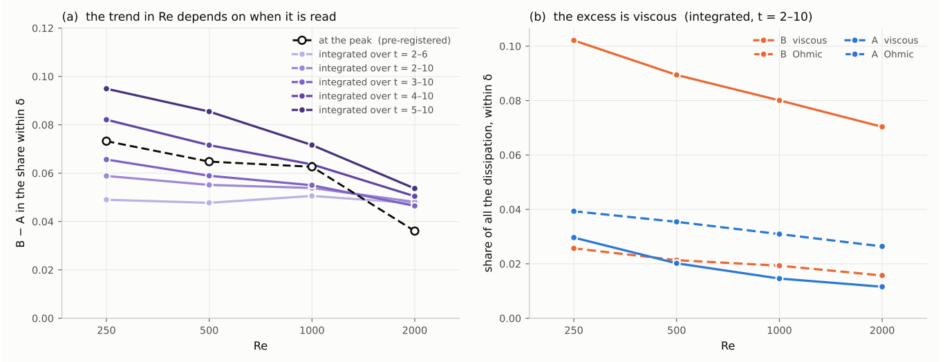
FIG. 2. (a) B-A in the share of the dissipation within \delta of the walls against Re : at the turbulent peak, as pre-registered (dashed), and integrated over five time windows, after the fact (light to dark: later windows). (b) The integrated share F_1 over t = 2-10 for A and B, divided into its viscous and Ohmic parts. Grid bands are at most 0.001, smaller than the symbols.
