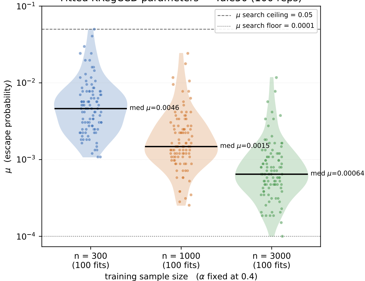
Fitted KRegCCD parameters — Yule50 (100 reps)
