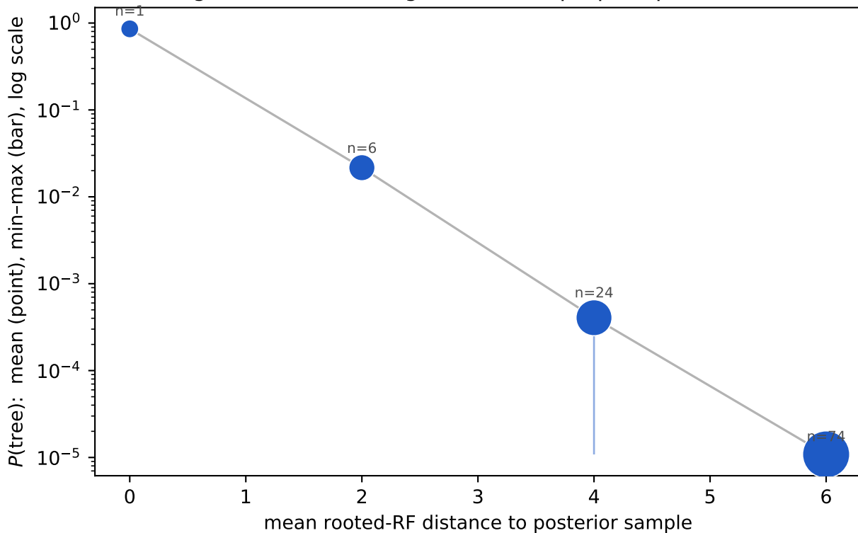
KRegCCD around a single tree: P(T) propto \epsilon^{(RF/2)}
