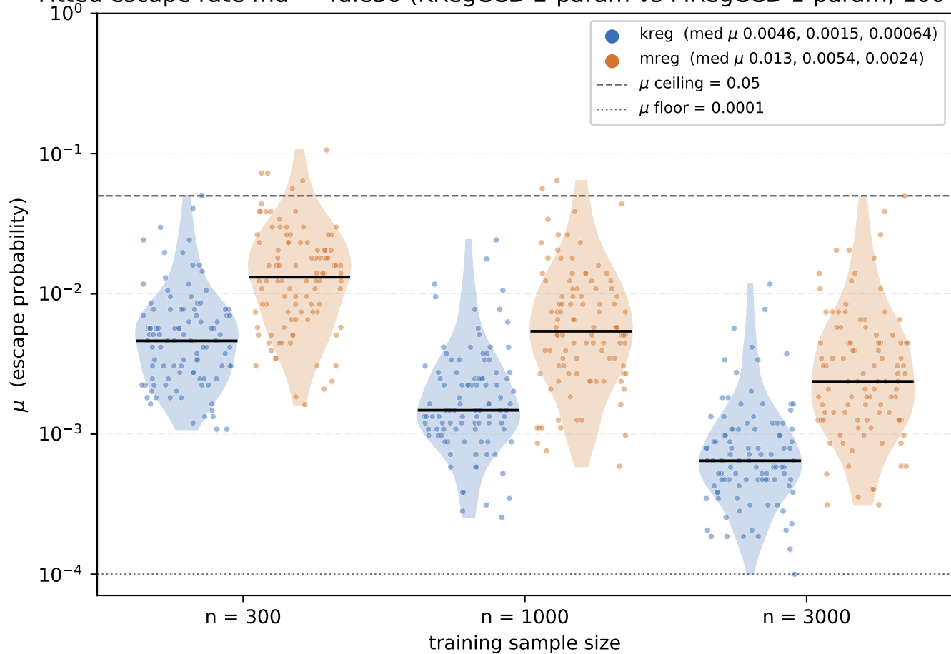
Fitted escape rate \mu — Yule50 (KRegCCD 2-param vs MRegCCD 1-param, 100 re
