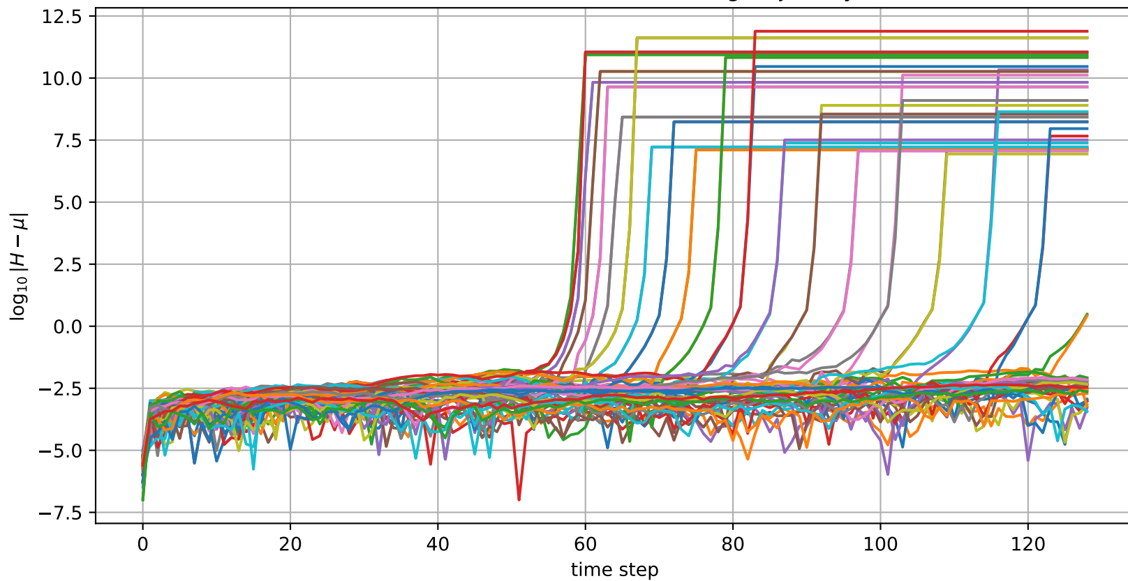
Hamiltonian conservation along trajectory
