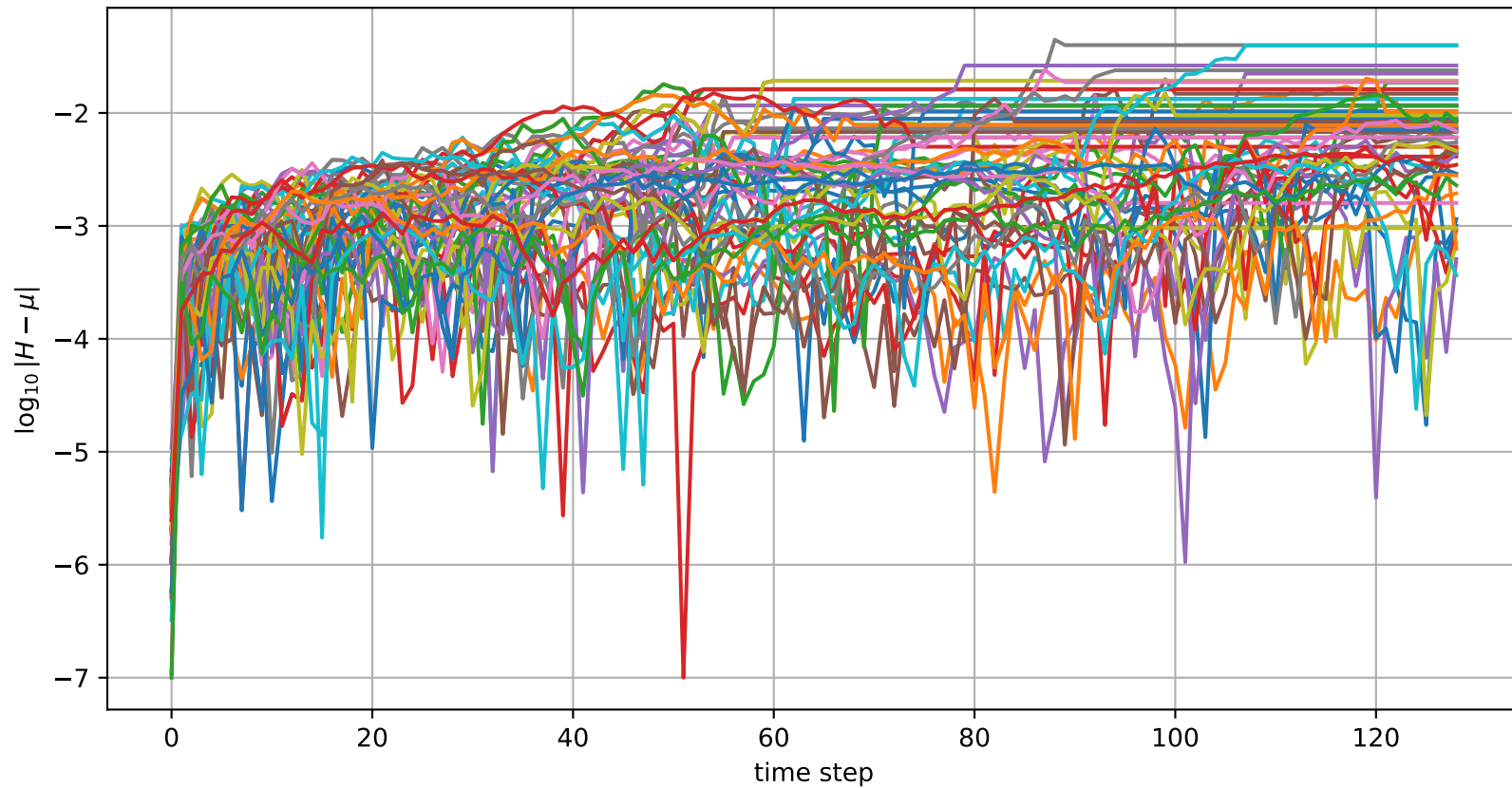
Hamiltonian conservation along trajectory
