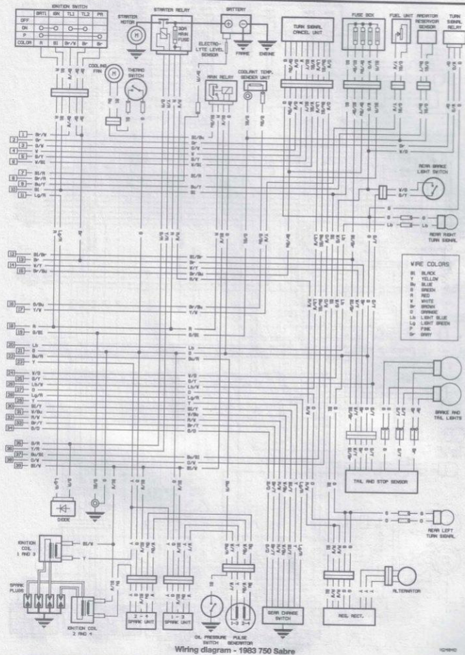
Wiring diagram - 1983 750 Sabre
