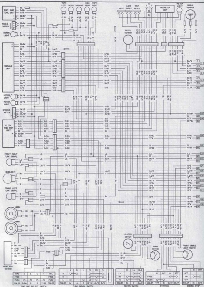
Wiring diagram - 1983 750 Sabre
