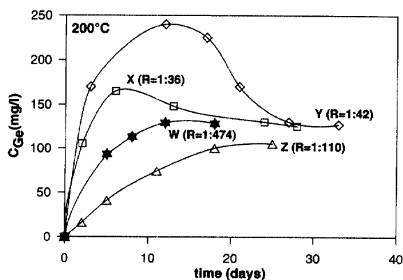
Fig. 2. Ge concentrations measured at 200°C as a function of time in neutral solutions in the dissolution runs of pretreated \text{GeO}_2(\text{tetr}) (see text) at different solid/solution ratios (R). The letters refer to the runs reported in Table 1. It can be seen that all the runs yield approximately the same steady-state aqueous Ge concentrations.
