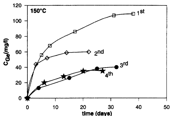
Fig. 1. Germanium concentrations measured at 150°C as a function of time in four successive \text{GeO}_2(\text{tetr}) dissolution runs in neutral ( 4 < \text{pH} < 6 ) solutions with solid/solution ratios from 1:50 to 1:30. The 3rd and 4th runs correspond to the runs N and O, respectively, listed in Table 1. It can be seen that Ge steady-state concentration values measured in the 3rd and 4th runs are approximately the same.
