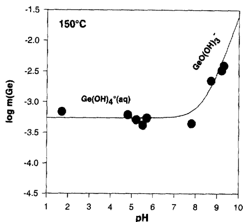
Fig. 4. Logarithm of \text{GeO}_2(\text{tetr}) solubility as a function of pH at 150°C and P_{\text{sat}} . The curve was calculated using values of K_{\text{tetr}} and K_{\text{dis}} (reactions 1 and 3) generated in this study.
