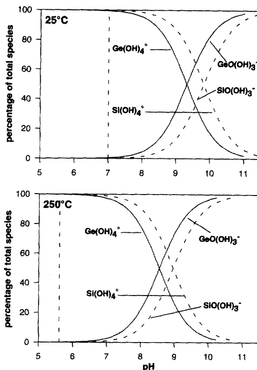
Fig. 6. Distribution of Ge and Si hydroxide species as a function of pH at 25 and 250°C, and P_{\text{sat}} . The distribution curves were calculated using the parameters given in Table 6 and in SUPCRT92 for Ge and Si aqueous hydroxide species, respectively. The vertical dashed lines stand for the pH of the neutrality point of water at a given temperature.
