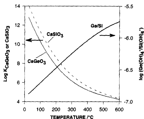
Fig. 7. Log K of \text{CaSiO}_3 (wollastonite) and \text{CaGeO}_3 (Eqns. 7 and 8), and of \text{Ge(OH)}_4^0/\text{Si(OH)}_4^0 ratio in a solution in equilibrium with a germanium-bearing wollastonite containing 1.4 ppm Ge as a function of temperature and at 1 kbar.
