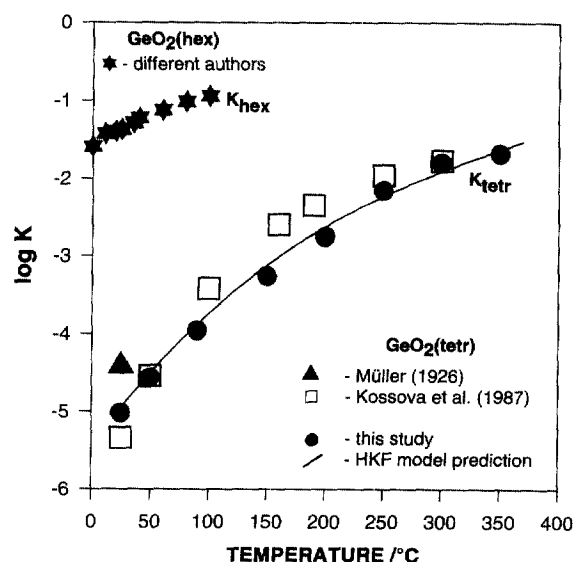
Fig. 3. Logarithms of \text{GeO}_2(\text{tetr}) and \text{GeO}_2(\text{hex}) dissociation constants as a function of temperature. The symbols were generated from experiments performed in this study (Table 2) and previous works (Table 3), but the curve was retrieved with the revised HKF model using the parameters given in Tables 5 and 6.
