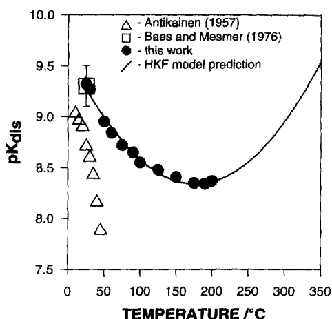
Fig. 5. Negative logarithm of germanic acid dissociation constant (reaction 3) as a function of temperature at P_{\text{air}} . The symbols depict experimental data generated in this work and taken from the literature, but the curve was retrieved with the revised HKF model using the parameters given in Tables 5 and 6.
