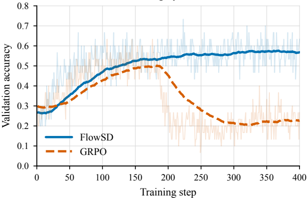
Training dynamics
