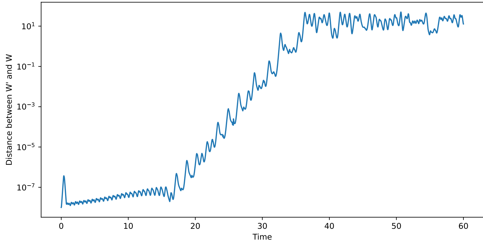
Divergence of Nearby Lorenz Trajectories
