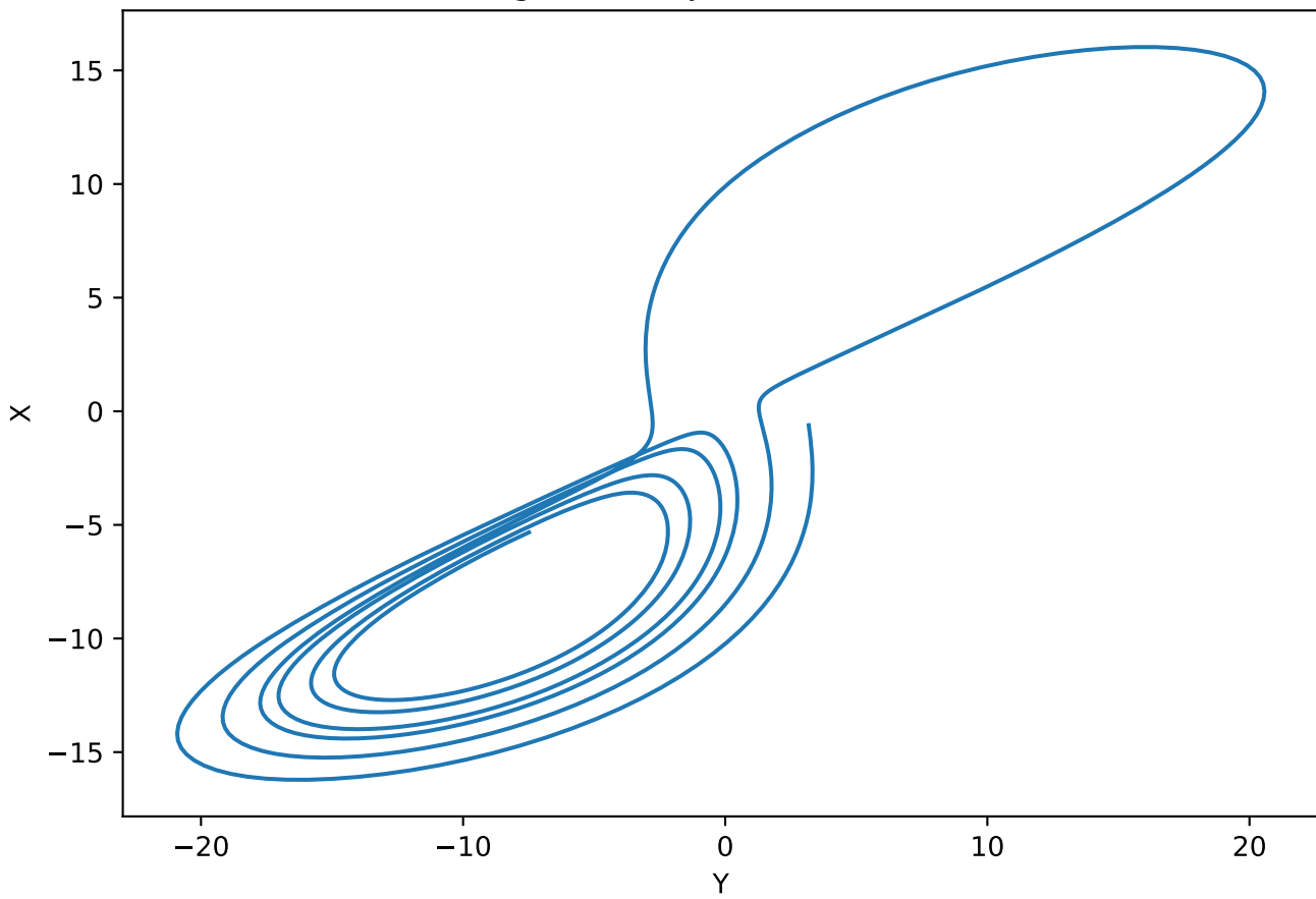
Lorenz Figure 2: Projection on the Y-X Plane
