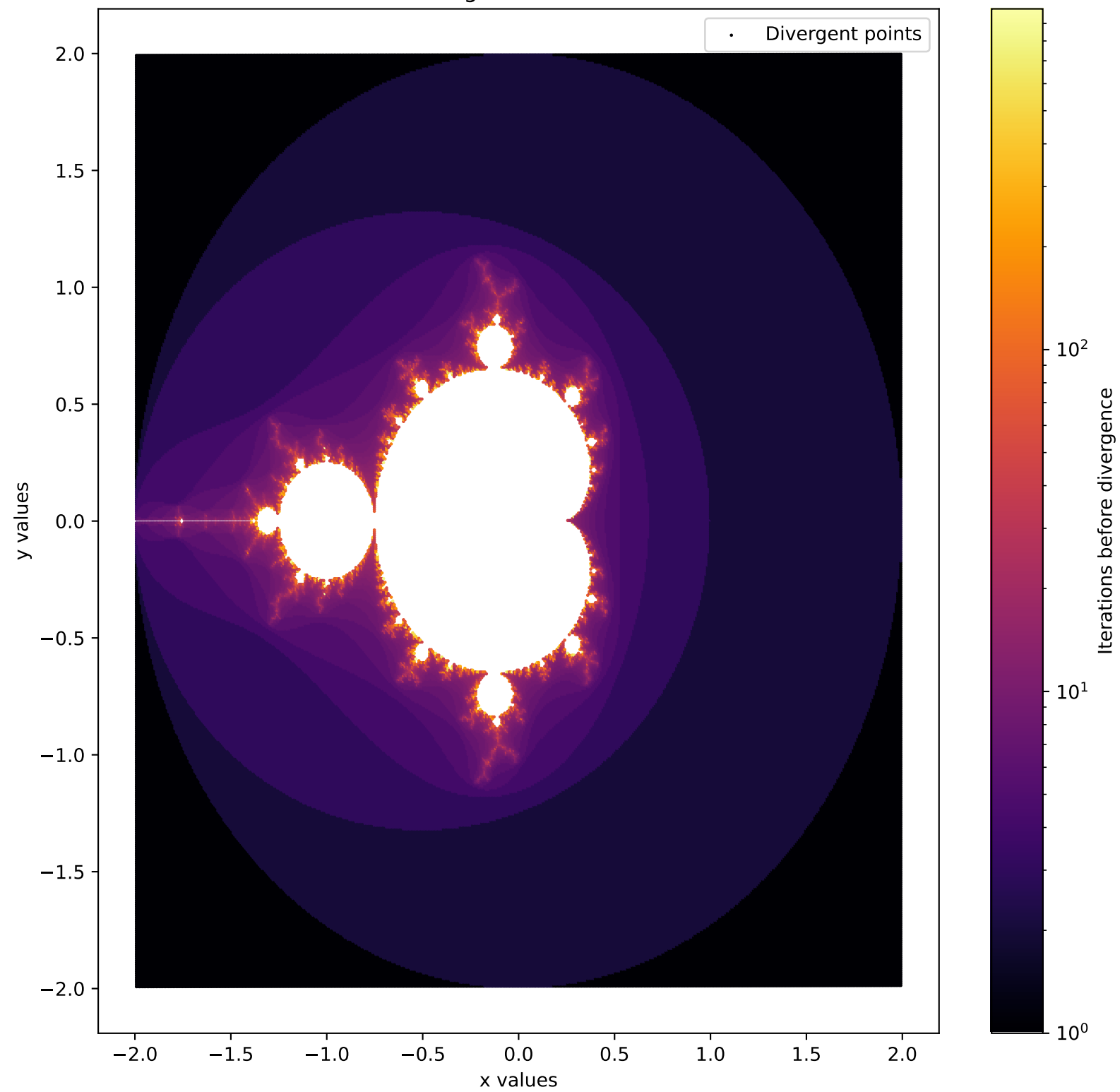
Iteration Count For Divergence for the Mandelbrot Iteration
