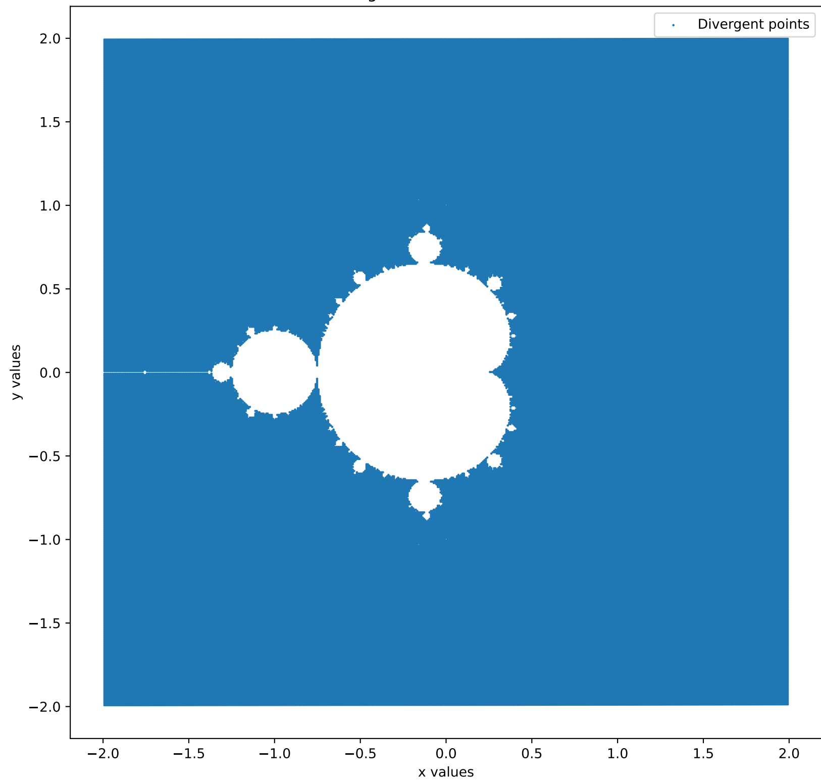
Bounded and Divergent Points of the Mandelbrot Iteration
