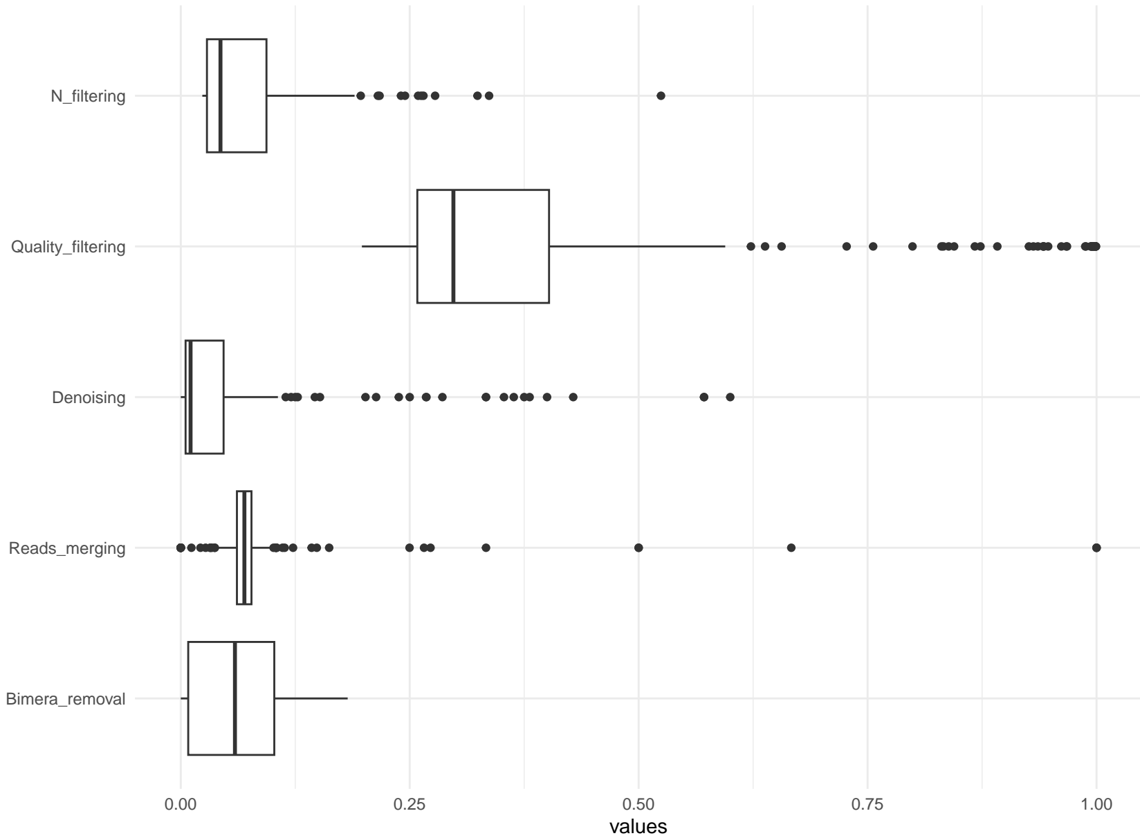
Proportion of reads lost at a specific pipeline step.
