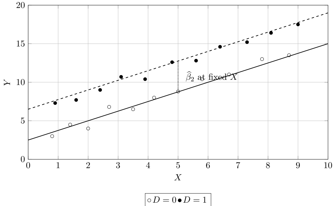
Figure 3.2: With no interaction, a binary predictor shifts the fitted line vertically while the slope on X remains the same. The coefficient on D is the vertical difference between predictions at the same X .
