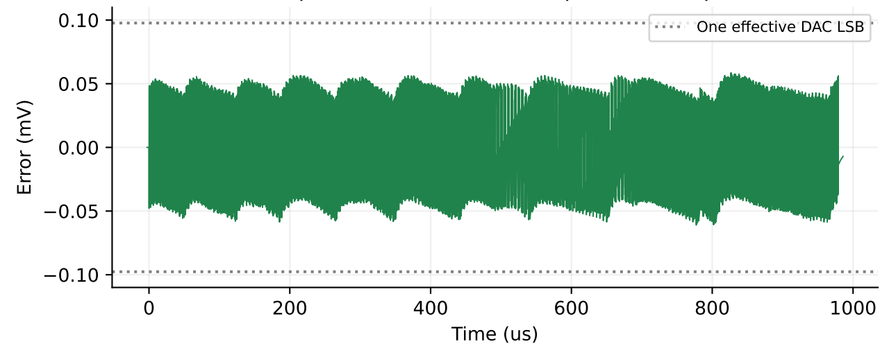
RC output error across all 100 points x 2 repeats
