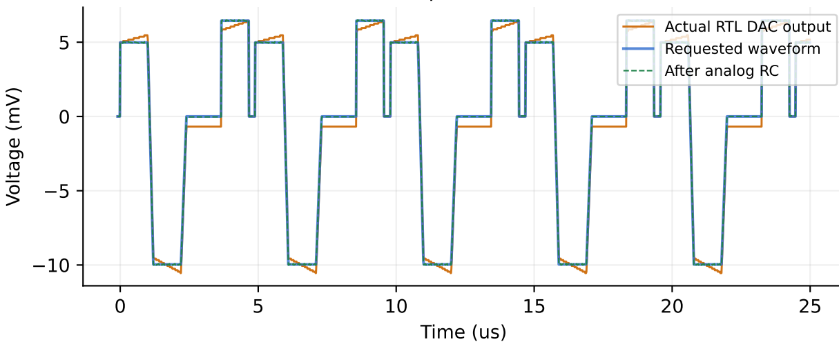
AWG output 2: DC + RC
