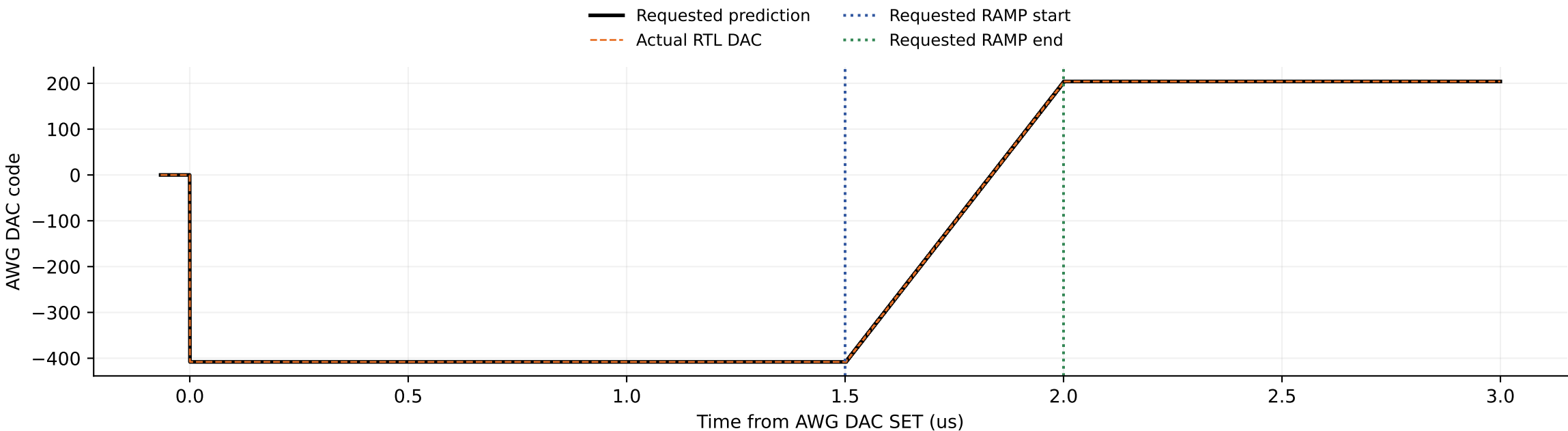
AWG timing: exact hold/ramp durations plus the fixed output-path latency
