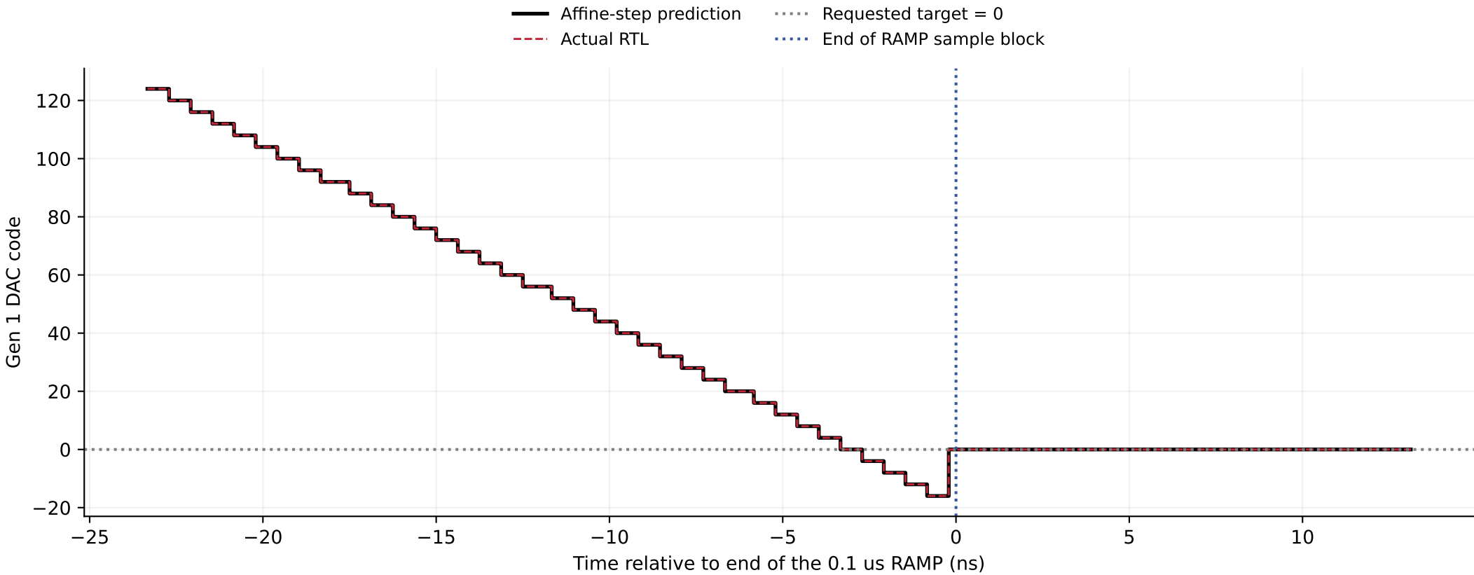
Observed undershoot at point (0,9): -16 codes = -0.390625 mV
