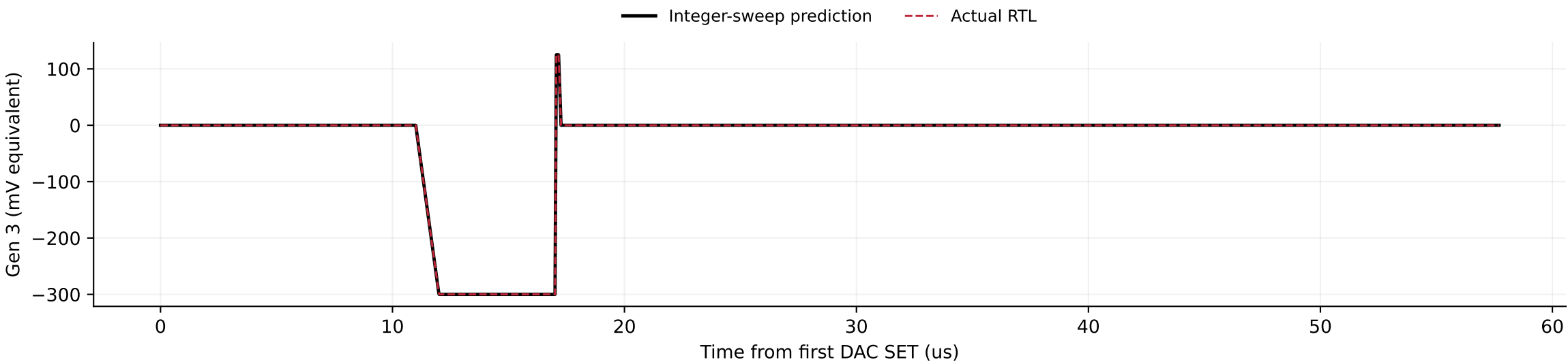
Screenshot waveform: actual two-channel RTL at the first sweep point Gen 3 set_3 = 125 mV; gen 1 set_3 = -75 mV; both channels checked on all 16 lanes
