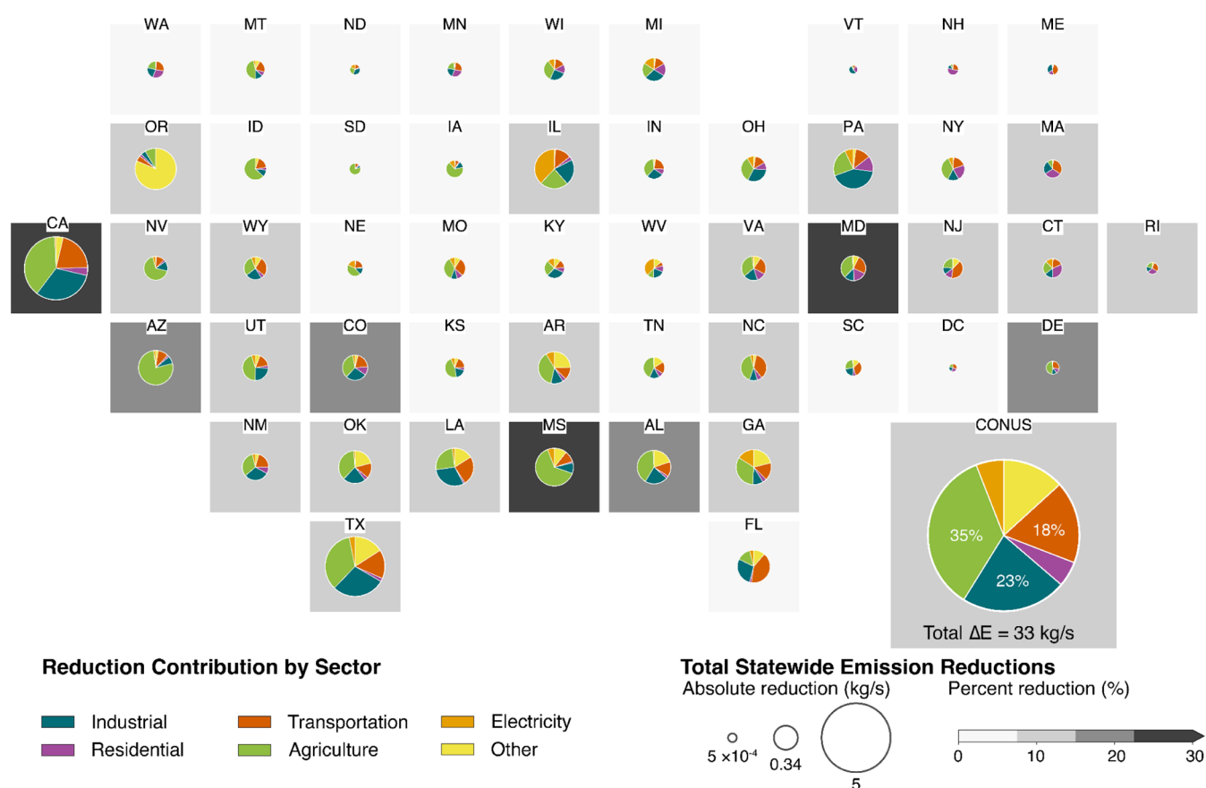
Figure 4. Sectoral emissions reductions required by the inverse model solution. Each tile represents state-level aggregate emission reductions. The pie-chart area scales with the absolute emissions reduction required in that state (kg/s); tile shading indicates the percent of emissions reduction relative to that state's baseline emissions. Wedge colors denote the sectoral contribution to each state's required reduction. A nationwide summary is shown at the bottom right. Equal-sized pies are shown in Figure S20.
