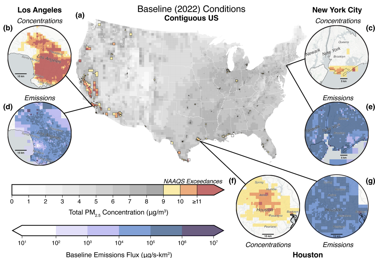
Figure 2. Baseline 2022 \text{PM}_{2.5} concentrations and emissions across the contiguous US demonstrate national heterogeneity in air pollution. Results are shown on a variable-resolution grid, with finer grid cells in more densely populated areas. (a) Gray tones denote concentrations below the annual \text{PM}_{2.5} NAAQS; outlined warm colors denote exceedances above 9 \mu\text{g}/\text{m}^3 , with darker tones indicating progressively higher concentrations. (b, c, f) Urban concentration insets for Los Angeles, New York City, and Houston, respectively. To highlight areas relevant to attainment, these insets show only grid cells exceeding 9 \mu\text{g}/\text{m}^3 . (d, e, g) Corresponding baseline (primary \text{PM}_{2.5} -equivalent) emissions fluxes aggregated across modeled anthropogenic sources, shown on a logarithmic scale for the same three cities.
