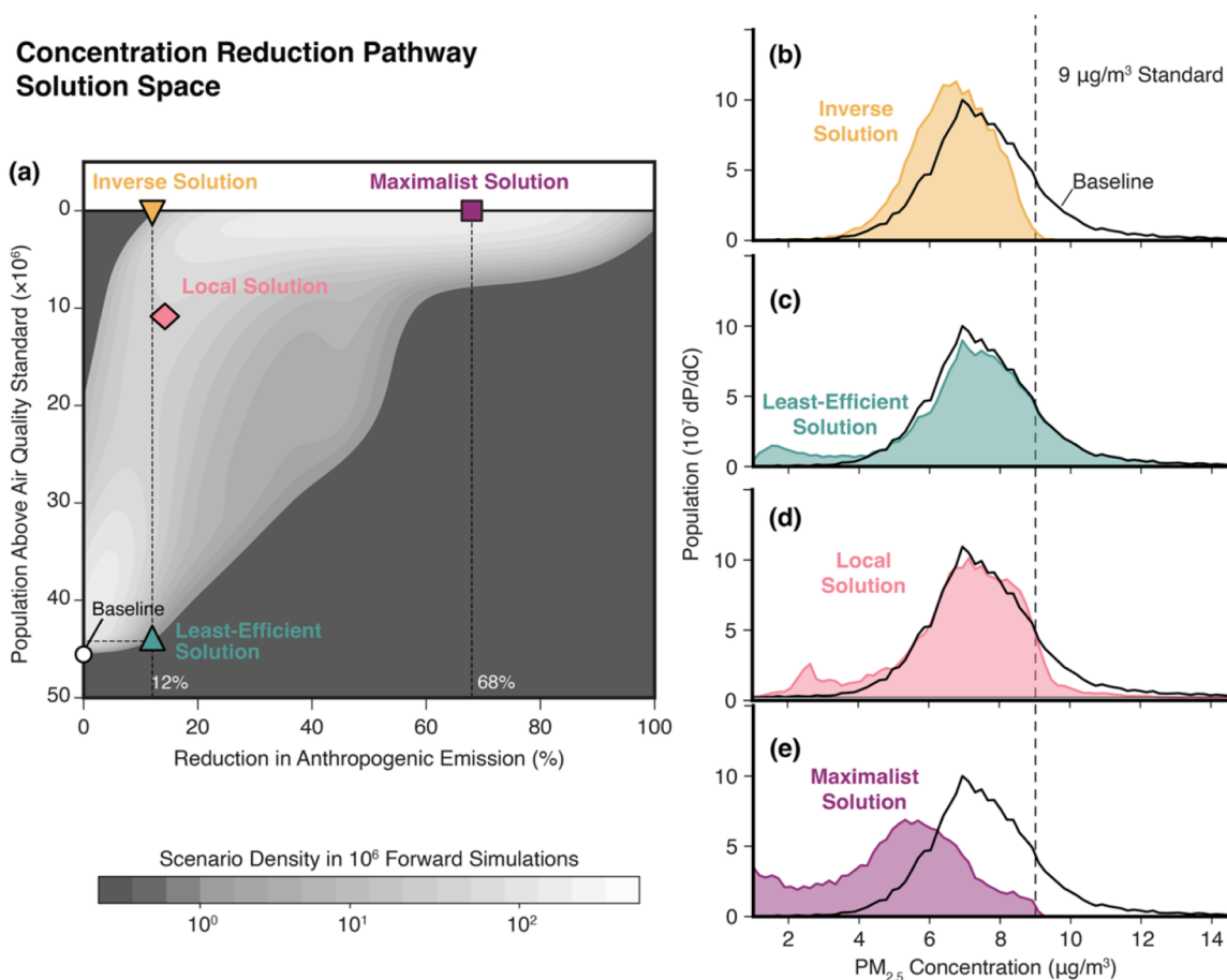
Figure 3. NAAQS compliance occupies a narrow efficient frontier in emissions-control space. (a) Density of 10^6 forward simulations in the space of total anthropogenic emissions reduction and population remaining above the annual health-based PM_{2.5} standard. Each simulated point represents a distinct spatial-sectoral-magnitude allocation of emissions reductions. Contours summarize the density of scenarios occupying this space. The x-axis reflects reductions in controllable emissions only. Baseline conditions are represented as a white circle with black outline. The inverse solution (gold triangle) lies on the efficient frontier, achieving compliance at \sim 12\% aggregate emissions reduction. Three additional scenarios represent poor spatial and sectoral allocation (teal triangle: “Least Efficient Solution”), a simple local reduction scheme (pink diamond: “Local Solution”), and brute-force heuristically chosen reductions (purple square: “Maximalist Solution”). (b–d) Population-weighted distributions of PM_{2.5} exposures for each scenario are compared to the baseline distribution and the annual NAAQS (dashed vertical line).
