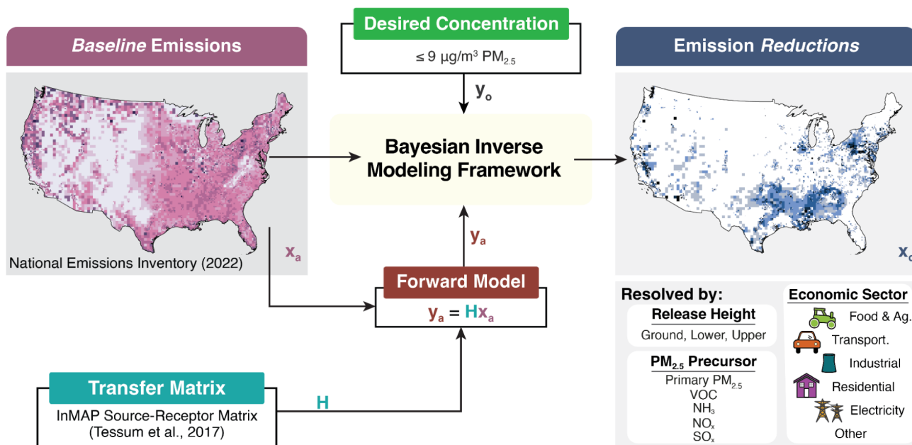
Figure 1. Model framework. We start from the baseline anthropogenic emissions field, x_a , and use the InMAP source-receptor matrix H to compute the corresponding baseline concentration field, y_a . The desired concentration end point, y_o , (here: annual-average PM_{2.5} concentrations at/below 9 \mu g/m^3 ) is imposed. Our model solves for a controlled emissions field, x_c , that satisfies the target while minimizing deviations from baseline emissions under physical and health-protective constraints. Results are resolved across space ( n = 54,111 ), five PM_{2.5} precursor species (primary PM_{2.5} , NO_x , NH_3 , VOC , and SO_x ) and six economic sectors.
