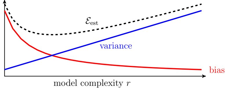
Figure 6.7: The estimation error \mathcal{E}_{\text{est}} incurred by linear regression can be decomposed into a bias term B^2 and a variance term V (see (6.22)). These two components depend on the model complexity r in an opposite manner resulting in a bias-variance trade-off.
