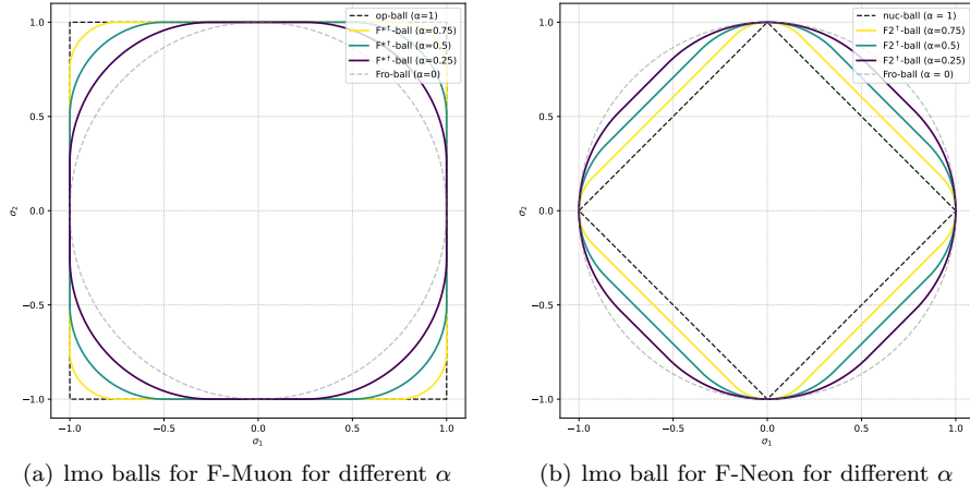
Fig. 8 Balls in the duals to F^* and F2 norms for different \alpha .
