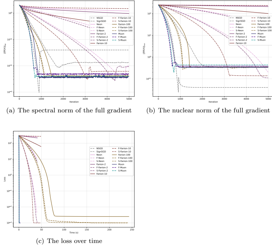
Fig. 10 More plots for the smooth convex problem (Equation (15)) for a 500x500 matrix.
