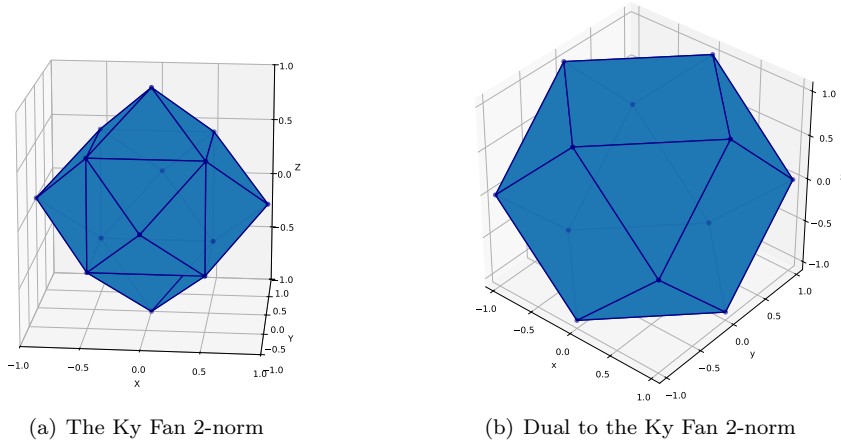
Fig. 9 Ky Fan 2-norm and its dual in the space of 3 singular values.
