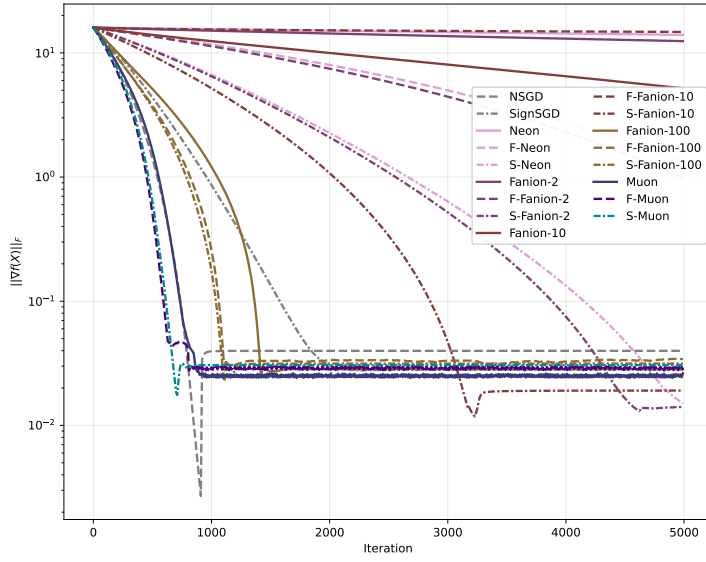
Fig. 1 A smooth convex problem (Equation (15)) for a 500x500 matrix.
