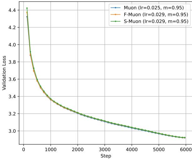
Fig. 5 The validation loss for GPT-2 Medium.
