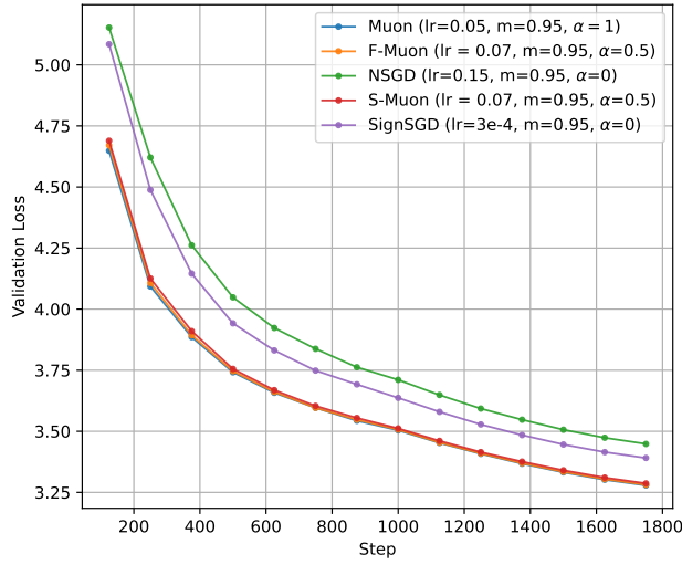
Fig. 4 The validation loss for NanoGPT.
