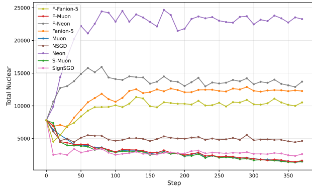
(c) Total nuclear norm
