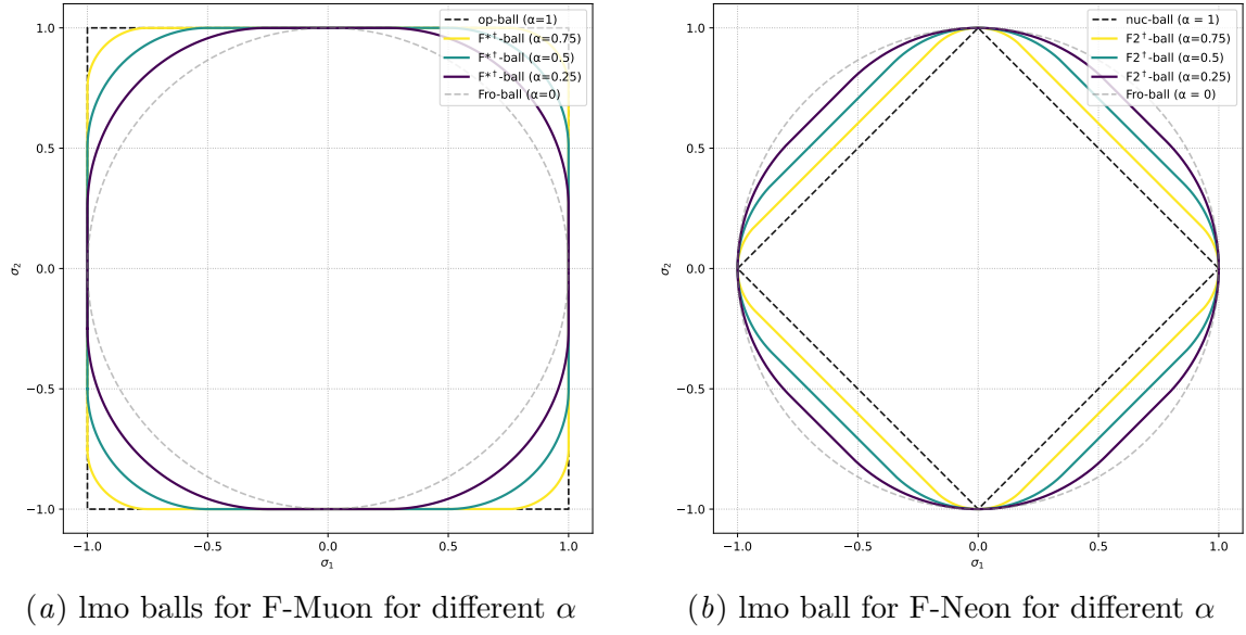
Figure 8: Balls in the duals to F^* and F_2 norms for different \alpha .
