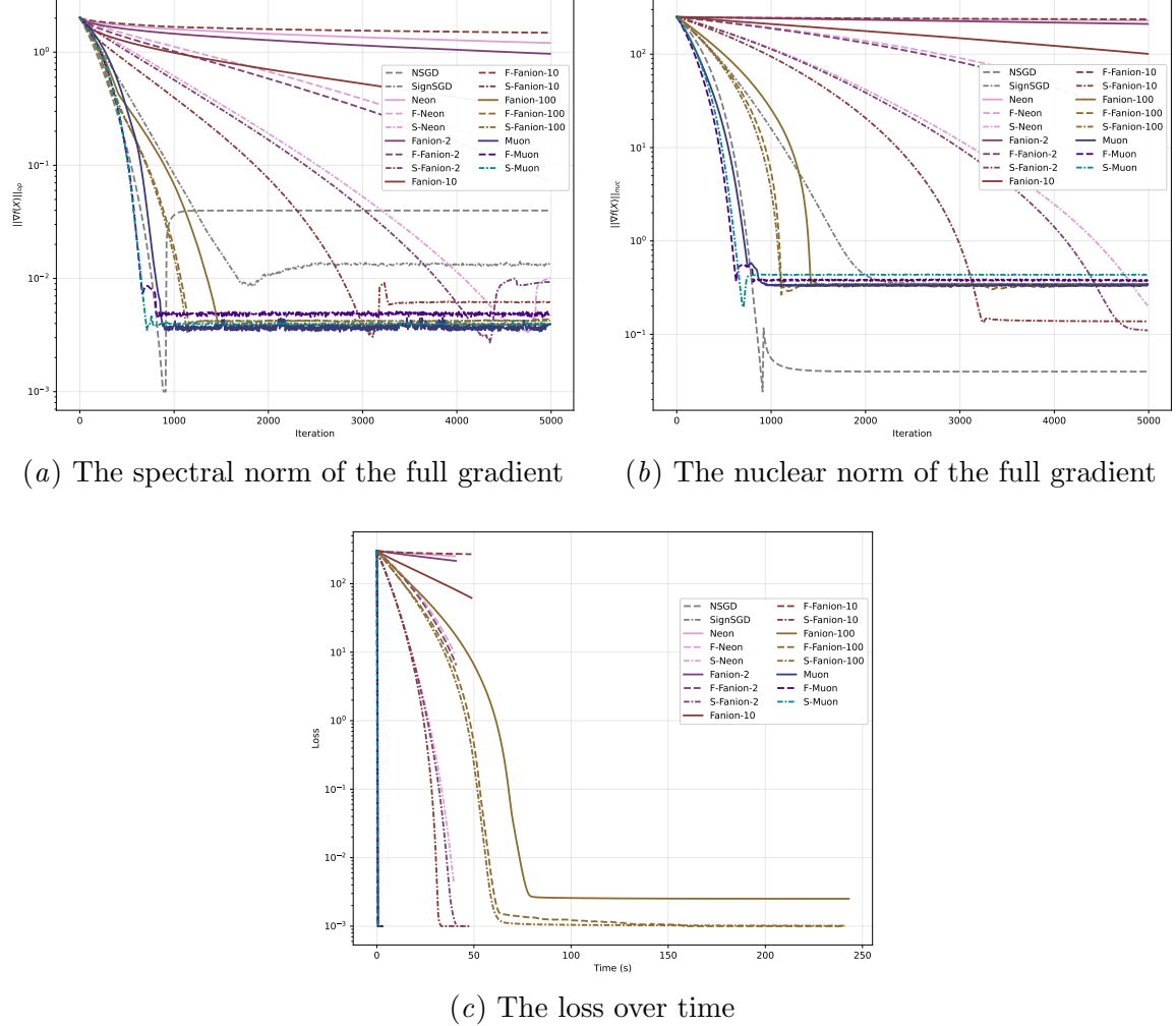
Figure 10: More plots for the smooth convex problem (Equation (15)) for a 500x500 matrix.
