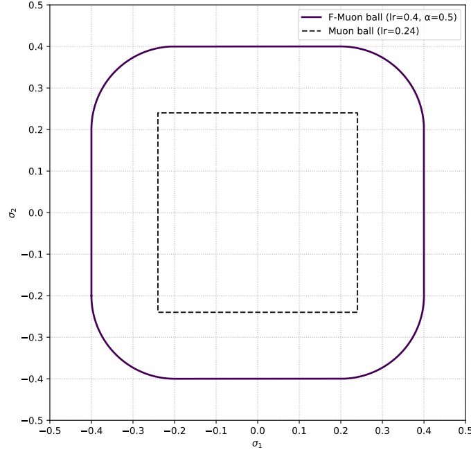
Figure 3: The LMO balls of Muon and F-Muon for training a CNN on CIFAR-10.
