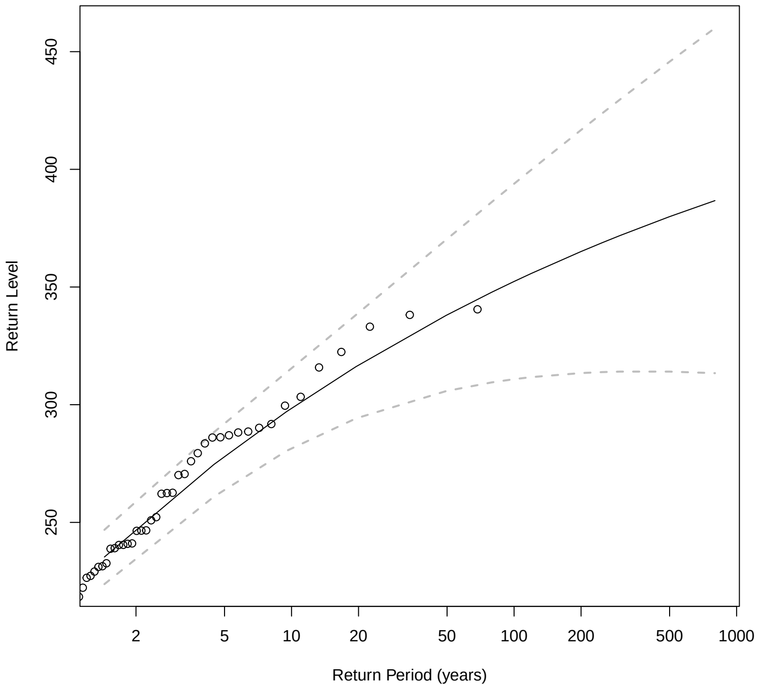
Stationary Return Level Curve: ADAMS
