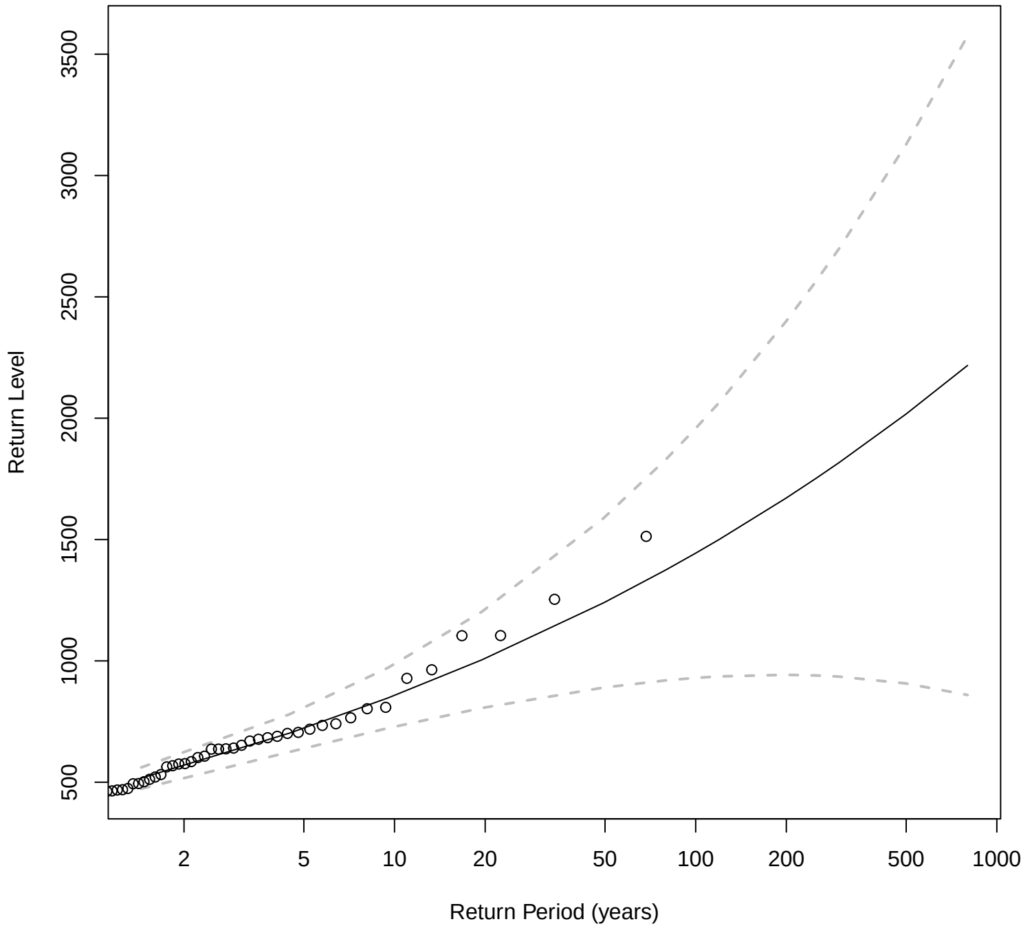
Stationary Return Level Curve: BCHSF
