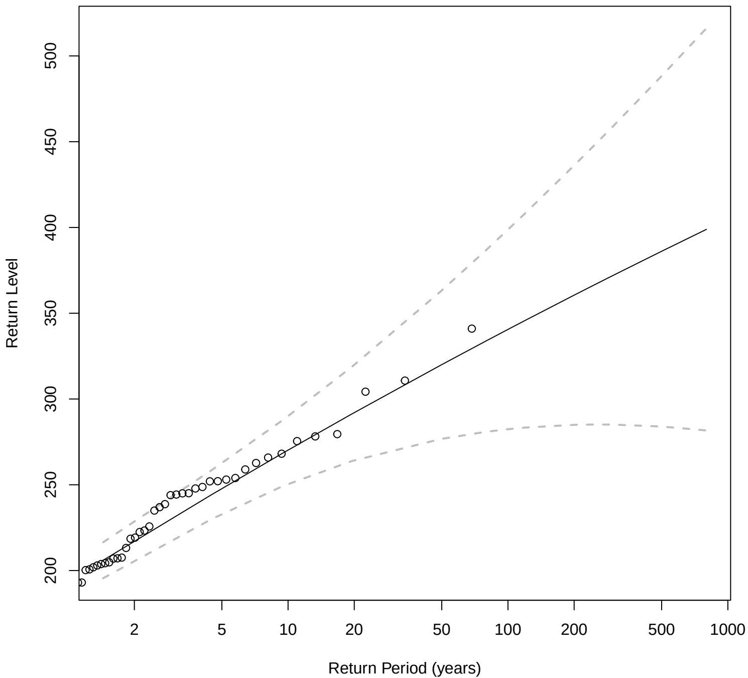
Stationary Return Level Curve: BCHLJ
