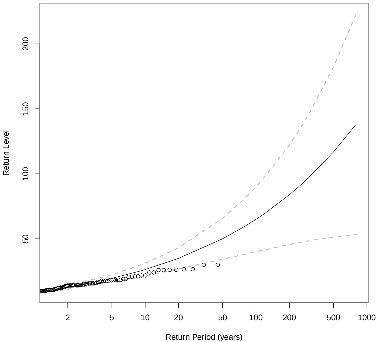
Stationary Return Level Curve: BAEZA
