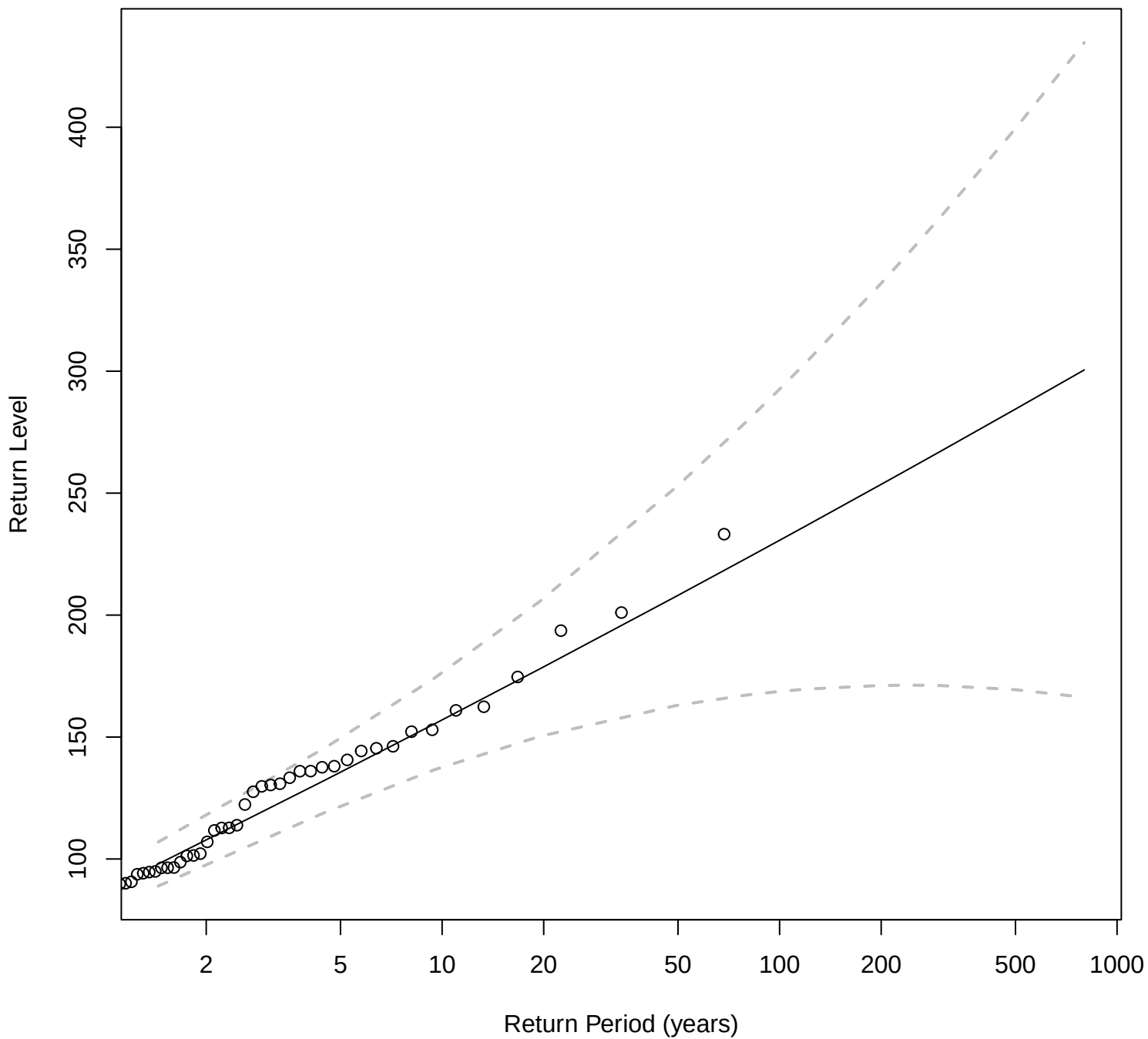
Stationary Return Level Curve: BCHAL
