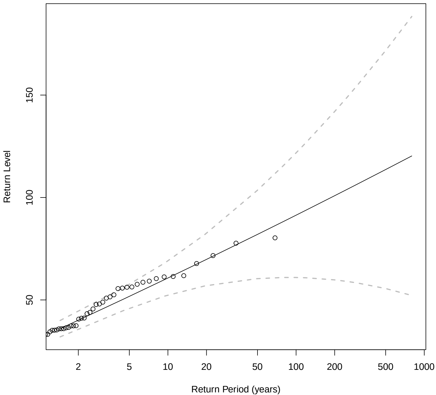
Stationary Return Level Curve: BAKER
