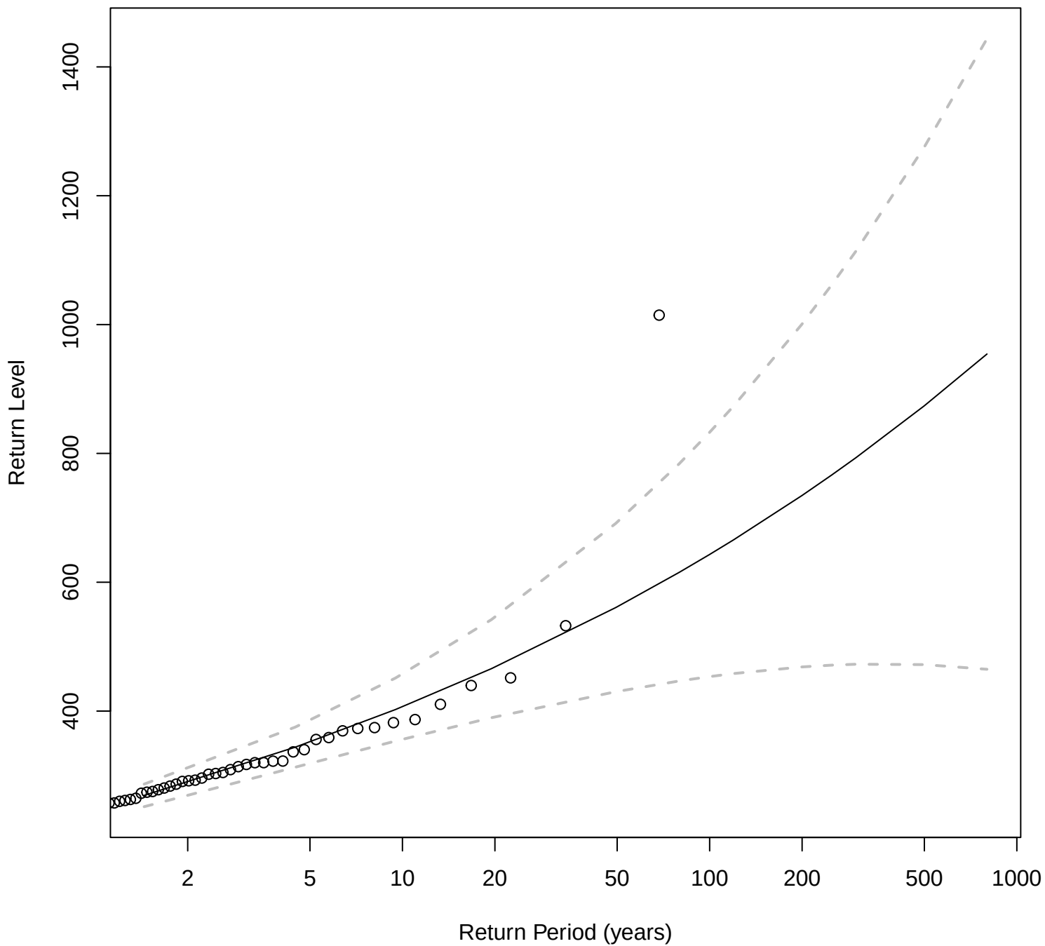
Stationary Return Level Curve: ARNT7
