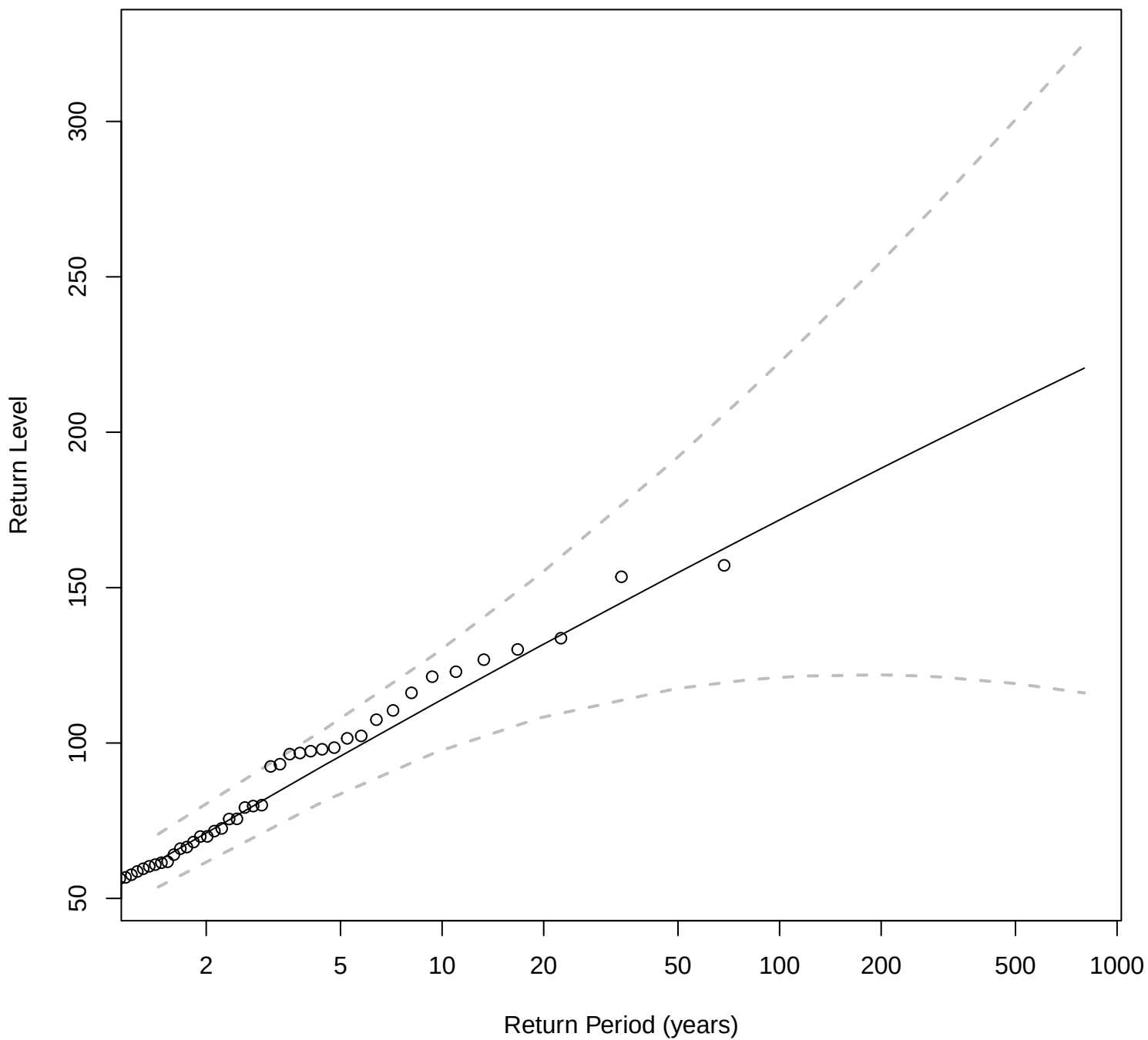
Stationary Return Level Curve: ASHNO
