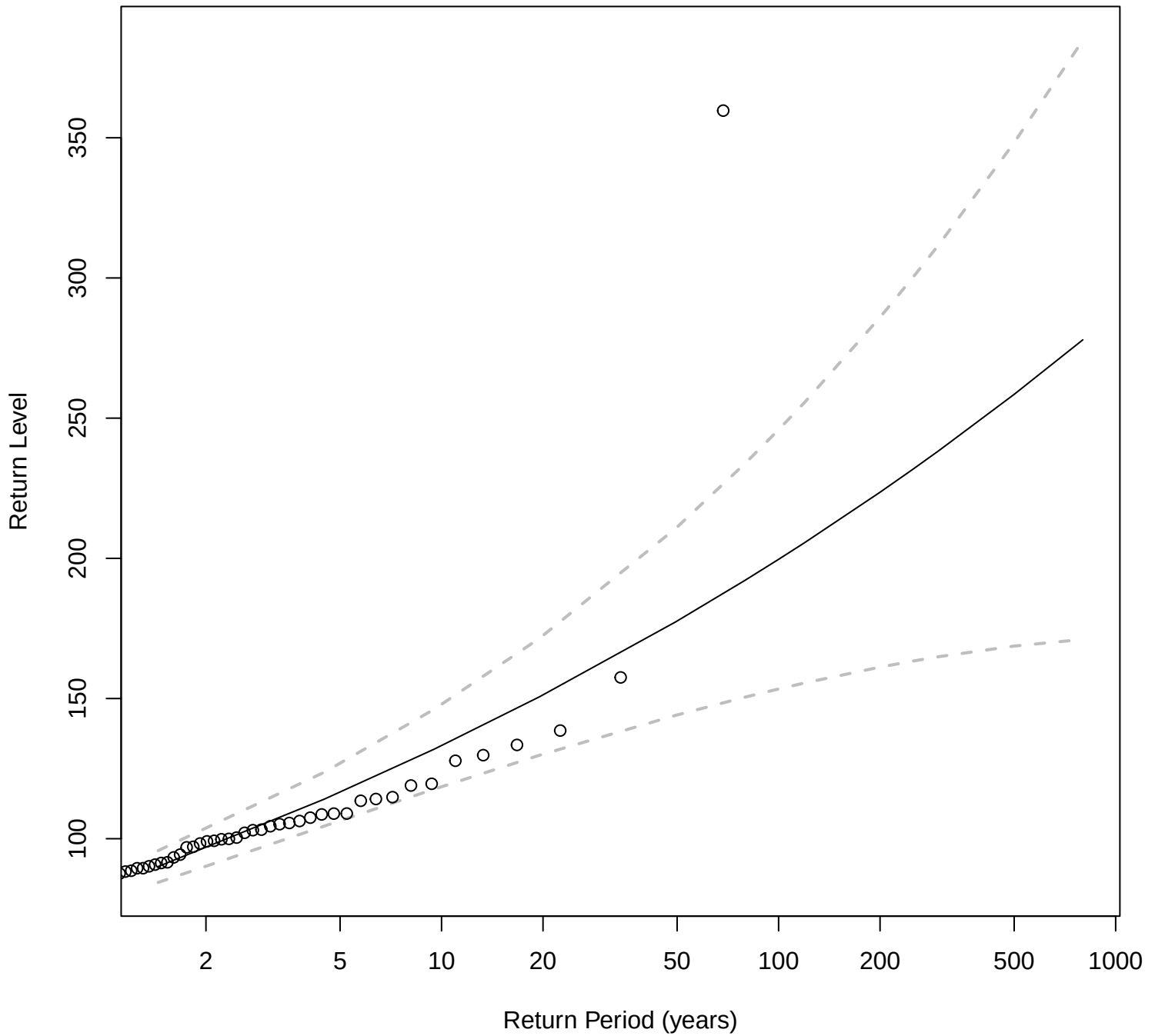
Stationary Return Level Curve: BARRM
