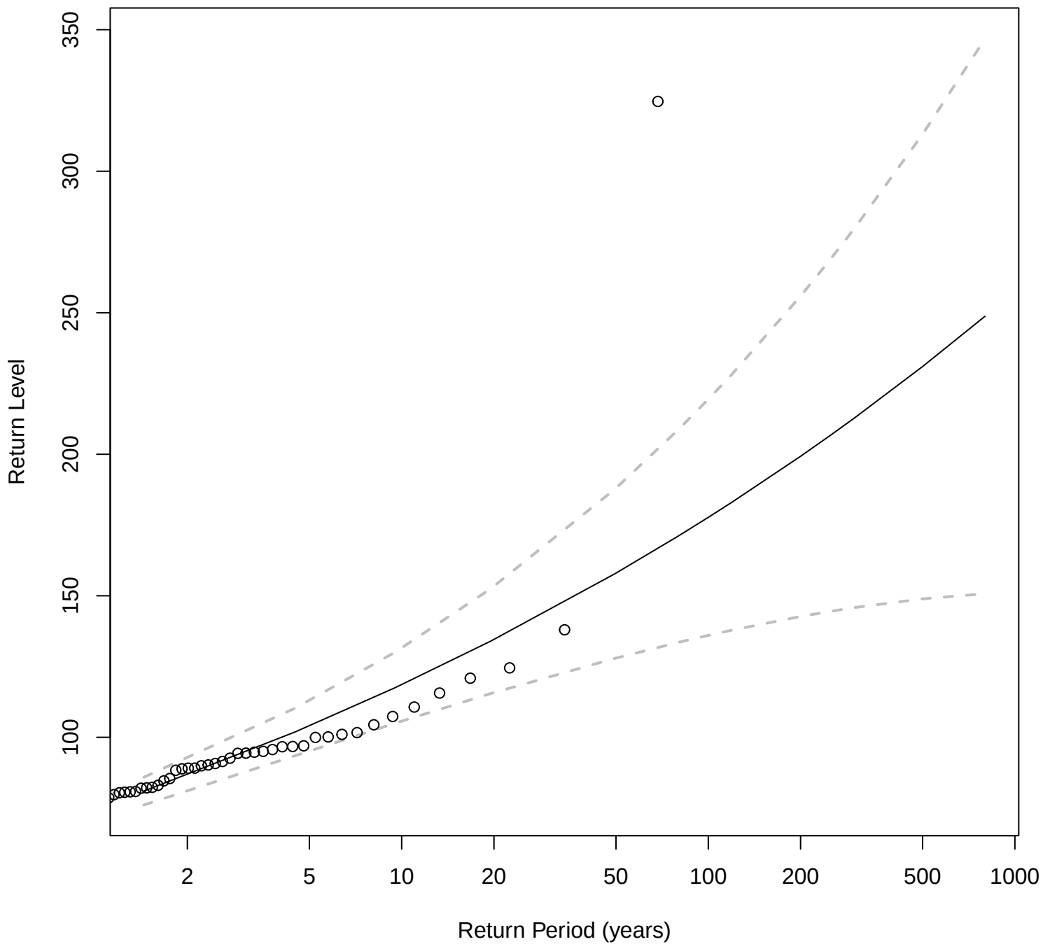
Stationary Return Level Curve: BARRS
