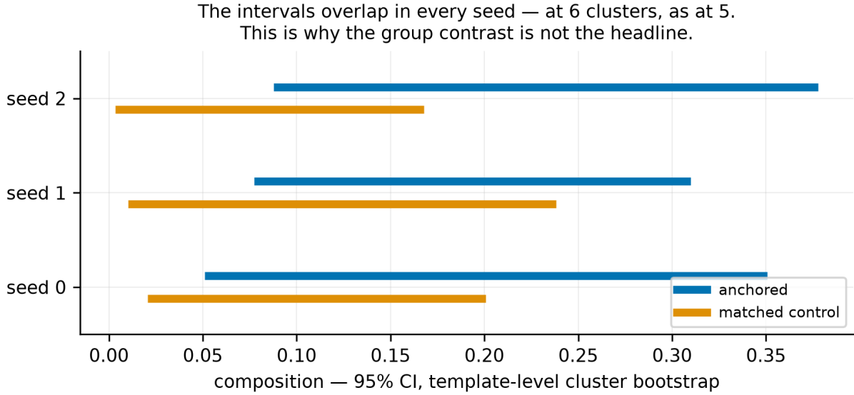
Figure 6: Template-level cluster bootstrap. The intervals overlap in every seed, at six clusters as at five.
