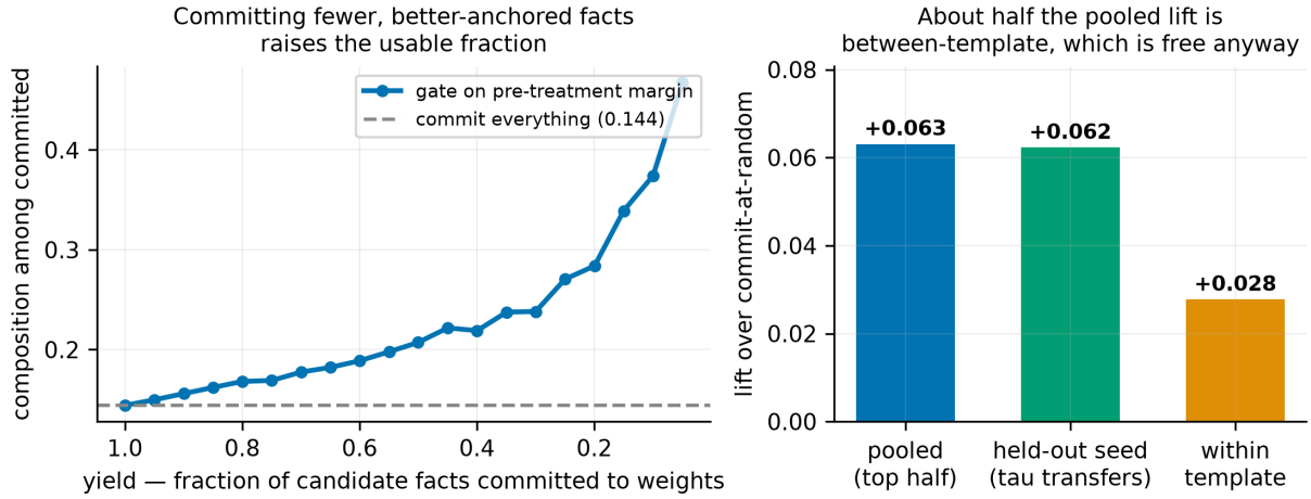
Figure 7: The commit/defer gate. Left: yield against composition among committed facts. Right: pooled, held-out and within-template lift.
