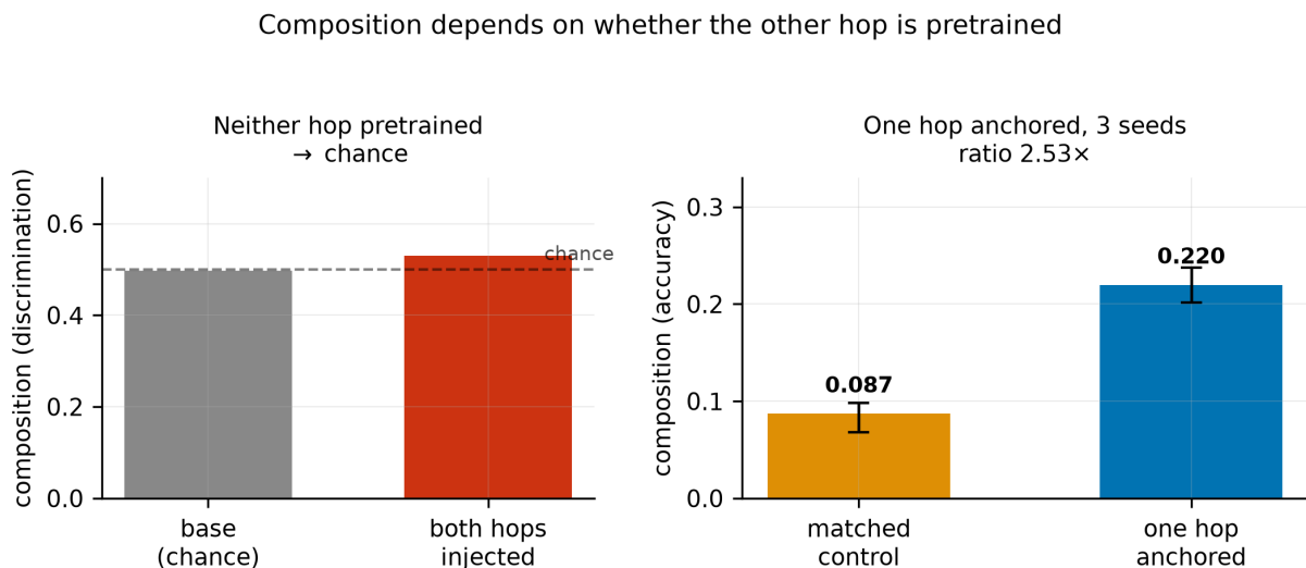
Figure 1: Composition by condition. With neither hop pretrained composition is at chance; with one hop anchored it separates from a matched control.
