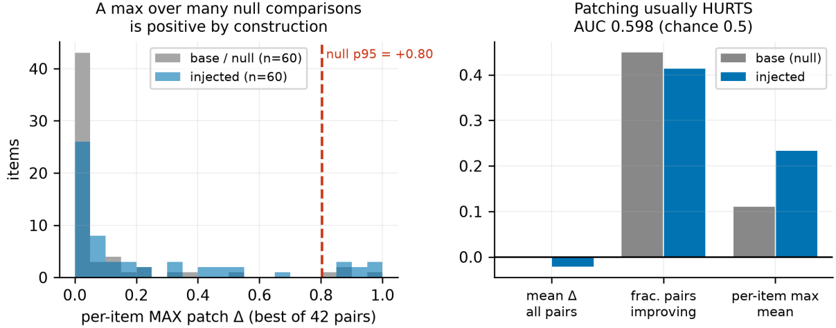
Figure 8: Self-patching against an appropriate null. A per-item maximum of +0.80 is what noise looks like on a model with nothing injected to relocate.
