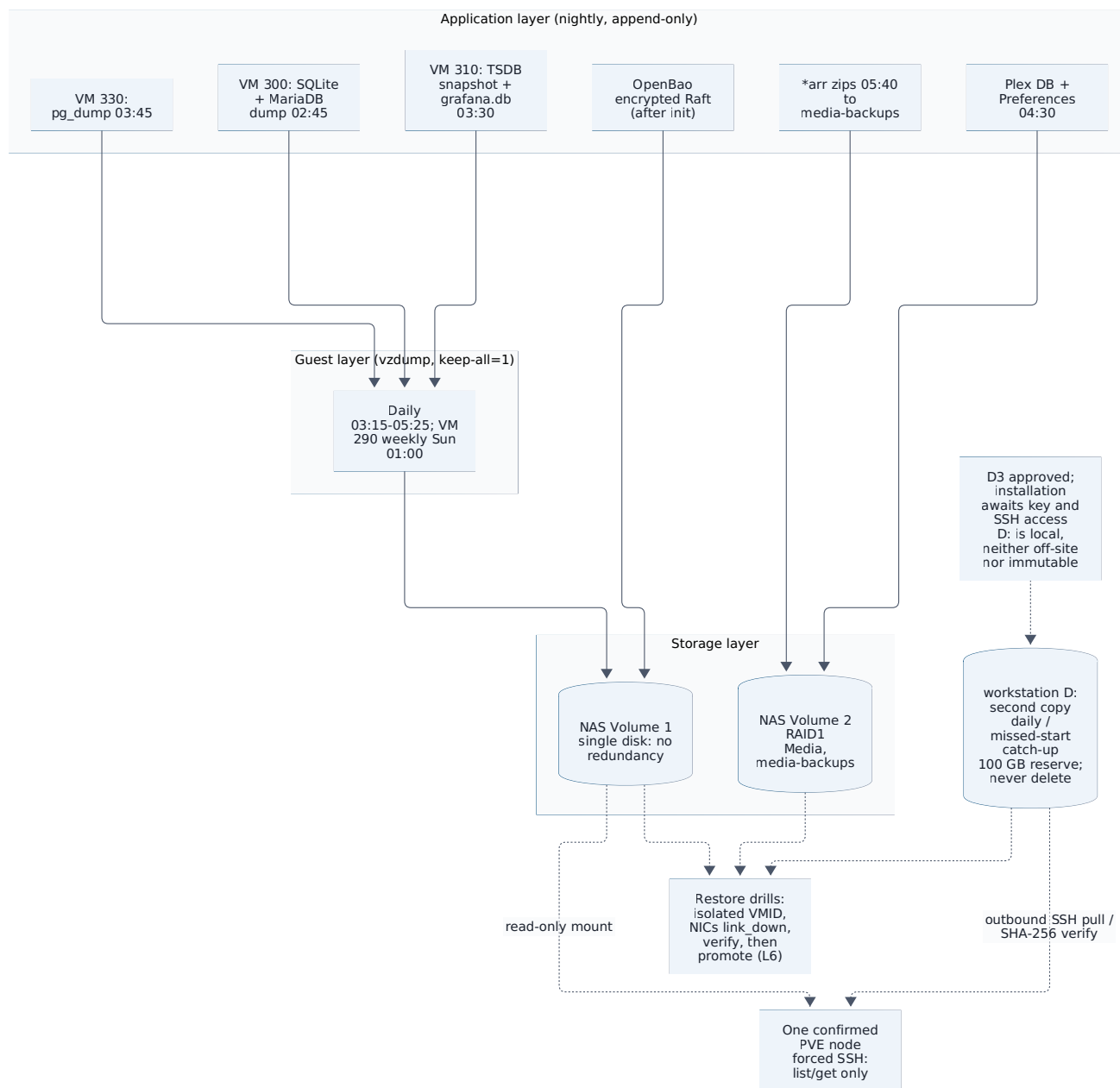
Figure 17. NAS backups, the approved read-only D: pull copy, and isolated restore paths
