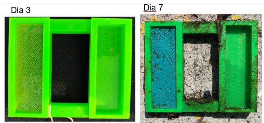
Detail of the corrosion effect on the copper mesh exposed to seawater. Copper chloride formation (blue-green coloring) is observed after 7 days of exposure. Each paired sample holder has a control and a sample (a slide without and with copper-mesh protection, respectively).
