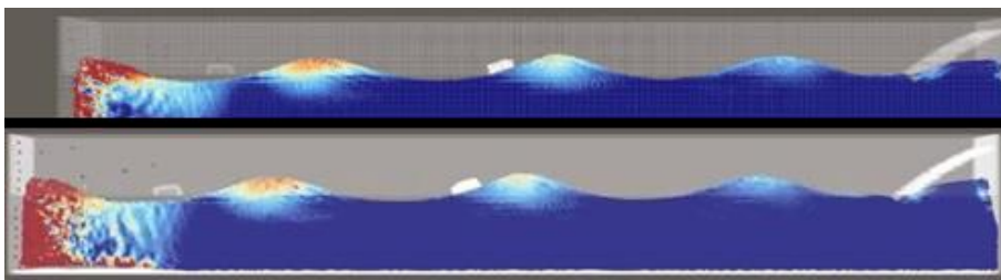
Wave-driven drift of scale cylinders: DualSPHysics simulations. Top: balanced cylinder. Bottom: unbalanced cylinder. In each image, the cylinder's initial position is shown on the left, and its position after a given time interval on the right.
