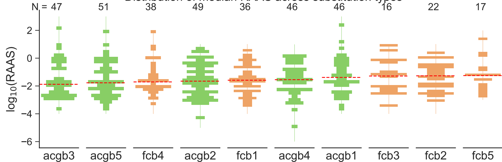
Distribution of median RAAS across substitution types
