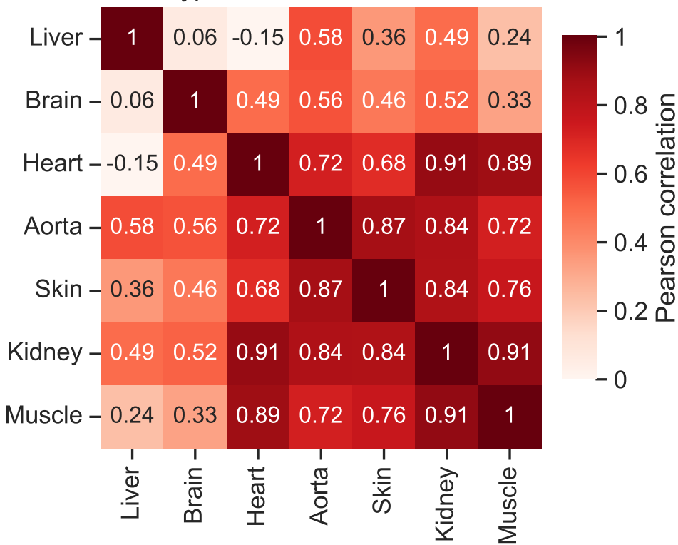
AAS type median RAAS correlation
